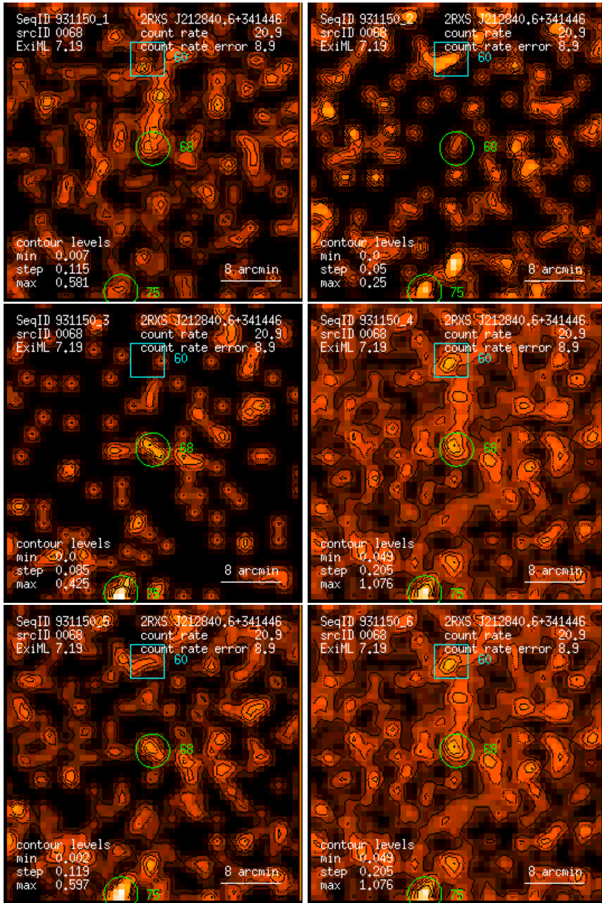
Figure 68: RASS 931150: detection 0068: band rate images, Gaussian filter: (1) PSPC channels 11 – 41, (2) 52 – 90, (3) 91 – 201, (4) 11 – 235, (5) 52 – 201, (6) 11 – 201. Broad band rates in counts/ks. Band rate contour levels in counts/ks/arcmin 2 .
