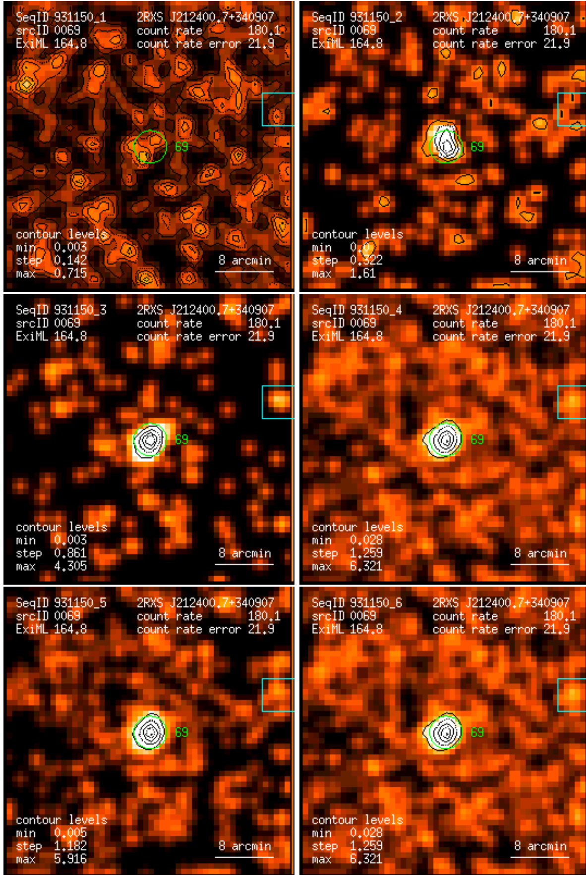
Figure 69: RASS 931150: detection 0069: band rate images, Gaussian filter: (1) PSPC channels 11 – 41, (2) 52 – 90, (3) 91 – 201, (4) 11 – 235, (5) 52 – 201, (6) 11 – 201. Broad band rates in counts/ks. Band rate contour levels in counts/ks/arcmin 2 .
