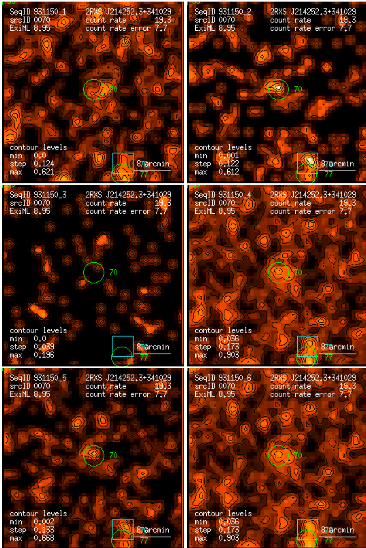
Figure 70: RASS 931150: detection 0070: band rate images, Gaussian filter: (1) PSPC channels 11 – 41, (2) 52 – 90, (3) 91 – 201, (4) 11 – 235, (5) 52 – 201, (6) 11 – 201. Broad band rates in counts/ks. Band rate contour levels in counts/ks/arcmin 2 .
