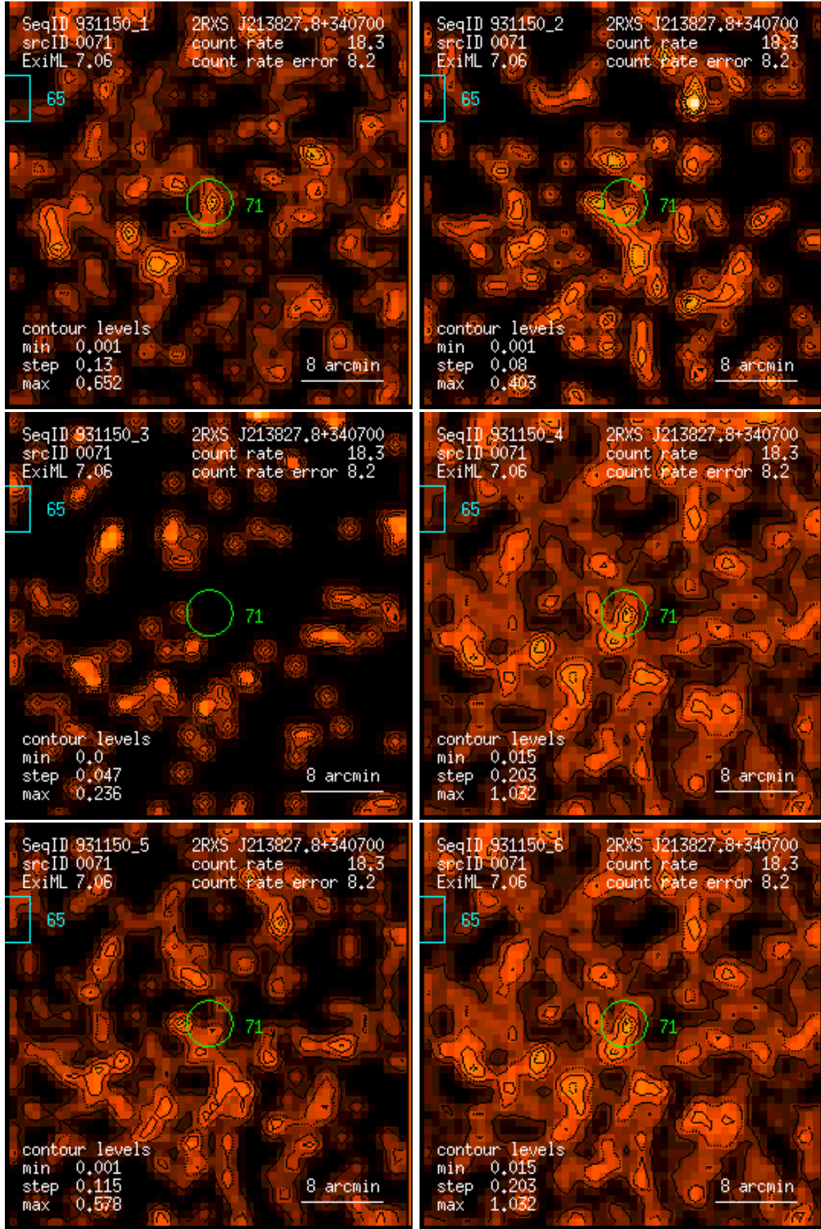
Figure 71: RASS 931150: detection 0071: band rate images, Gaussian filter: (1) PSPC channels 11 – 41, (2) 52 – 90, (3) 91 – 201, (4) 11 – 235, (5) 52 – 201, (6) 11 – 201. Broad band rates in counts/ks. Band rate contour levels in counts/ks/arcmin 2 .
