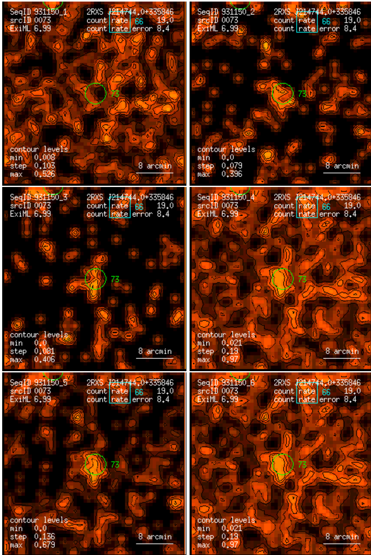
Figure 73: RASS 931150: detection 0073: band rate images, Gaussian filter: (1) PSPC channels 11 – 41, (2) 52 – 90, (3) 91 – 201, (4) 11 – 235, (5) 52 – 201, (6) 11 – 201. Broad band rates in counts/ks. Band rate contour levels in counts/ks/arcmin 2 .
