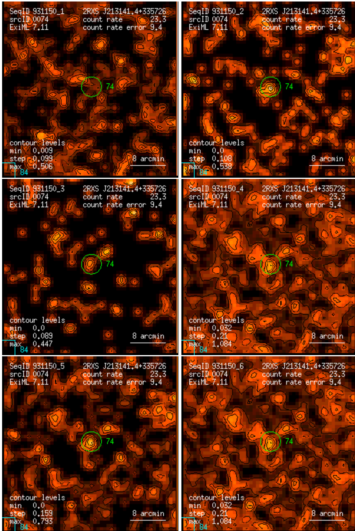
Figure 74: RASS 931150: detection 0074: band rate images, Gaussian filter: (1) PSPC channels 11 – 41, (2) 52 – 90, (3) 91 – 201, (4) 11 – 235, (5) 52 – 201, (6) 11 – 201. Broad band rates in counts/ks. Band rate contour levels in counts/ks/arcmin 2 .
