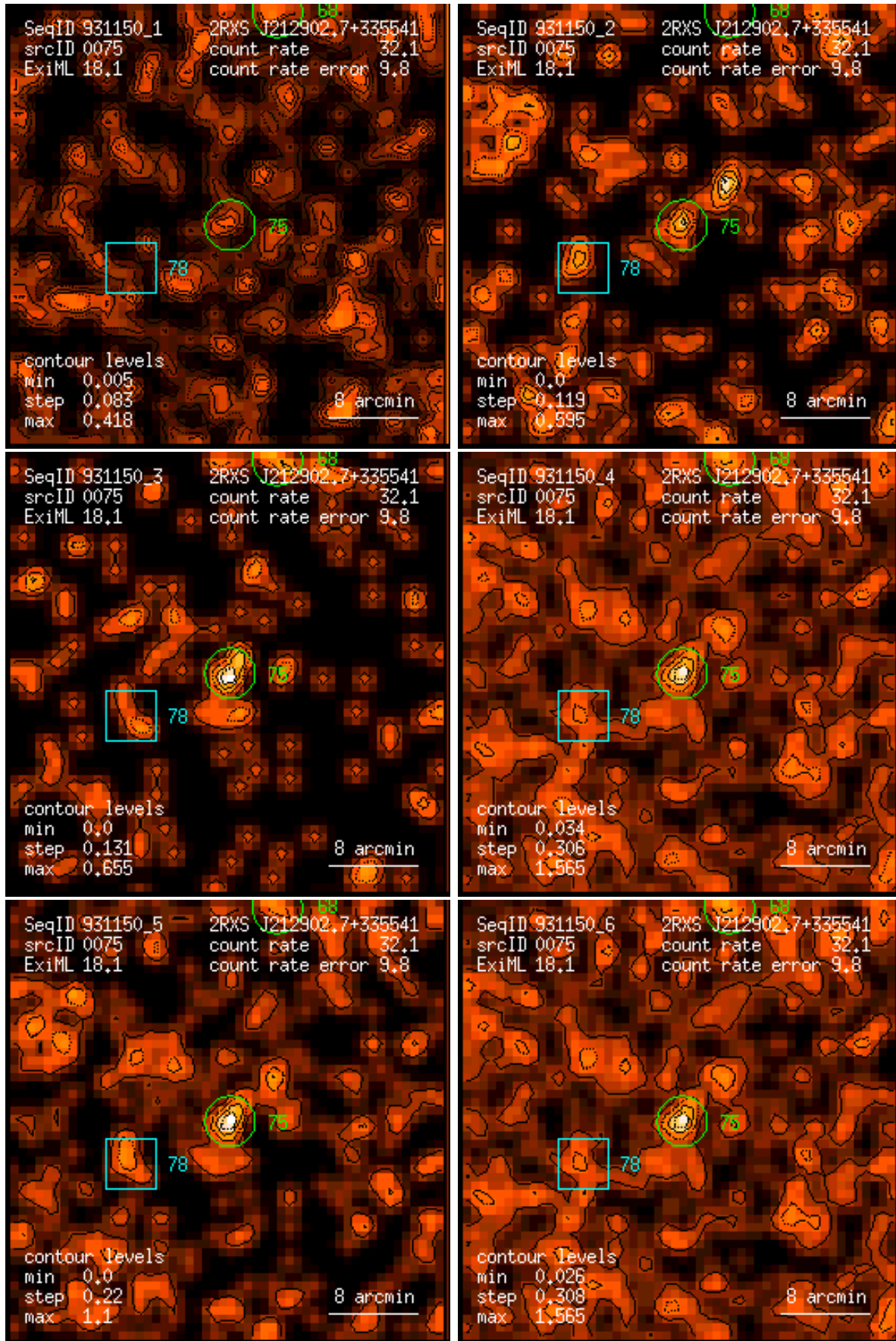
Figure 75: RASS 931150: detection 0075: band rate images, Gaussian filter: (1) PSPC channels 11 – 41, (2) 52 – 90, (3) 91 – 201, (4) 11 – 235, (5) 52 – 201, (6) 11 – 201. Broad band rates in counts/ks. Band rate contour levels in counts/ks/arcmin 2 .
