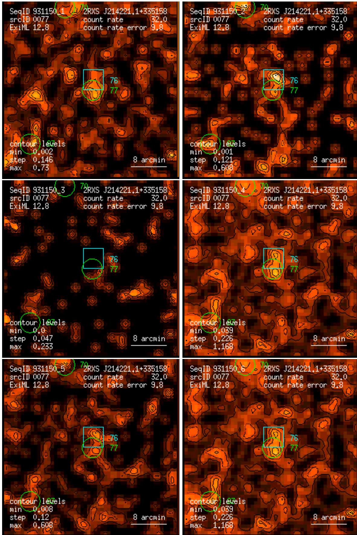
Figure 77: RASS 931150: detection 0077: band rate images, Gaussian filter: (1) PSPC channels 11 – 41, (2) 52 – 90, (3) 91 – 201, (4) 11 – 235, (5) 52 – 201, (6) 11 – 201. Broad band rates in counts/ks. Band rate contour levels in counts/ks/arcmin 2 .
