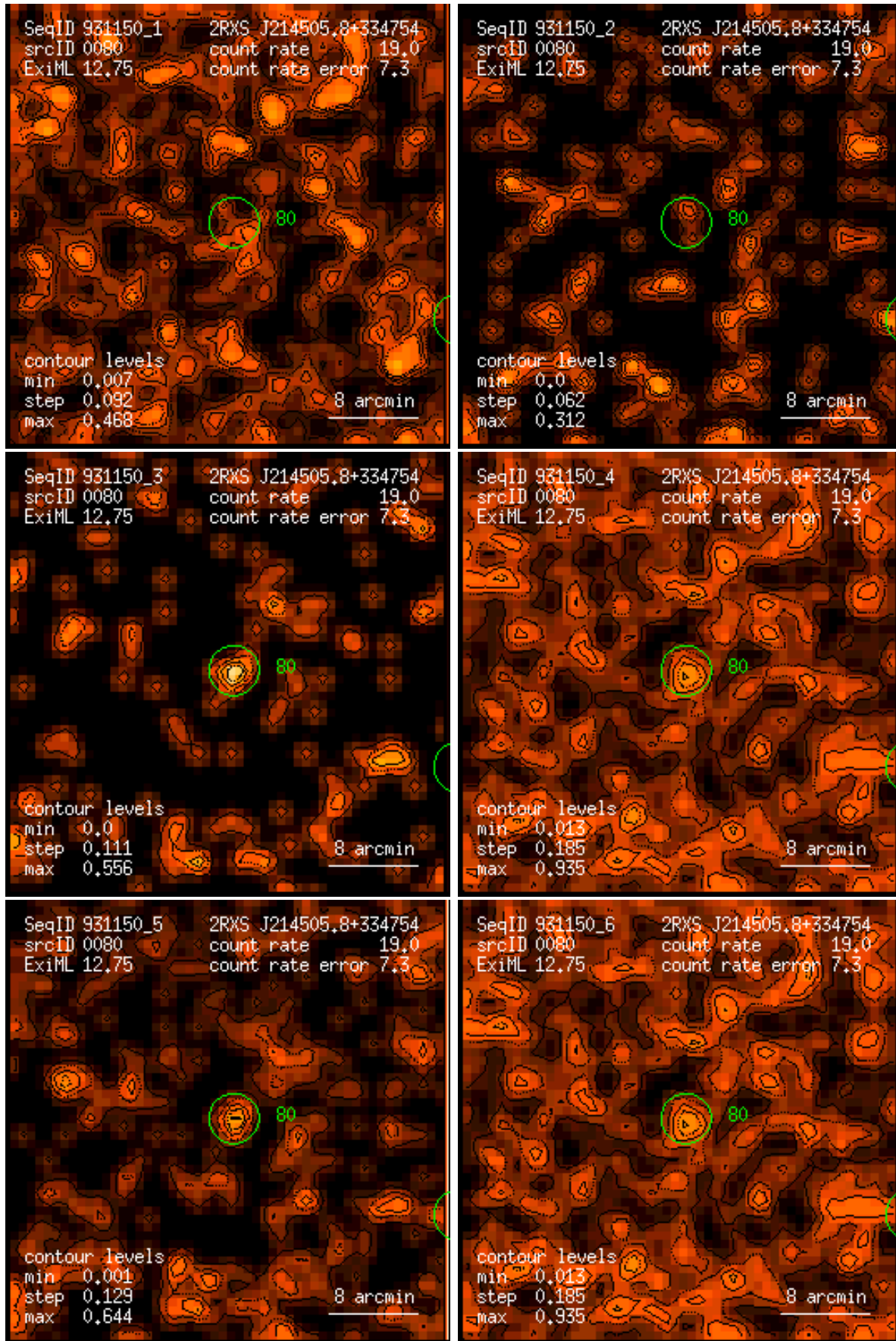
Figure 80: RASS 931150: detection 0080: band rate images, Gaussian filter: (1) PSPC channels 11 – 41, (2) 52 – 90, (3) 91 – 201, (4) 11 – 235, (5) 52 – 201, (6) 11 – 201. Broad band rates in counts/ks. Band rate contour levels in counts/ks/arcmin 2 .
