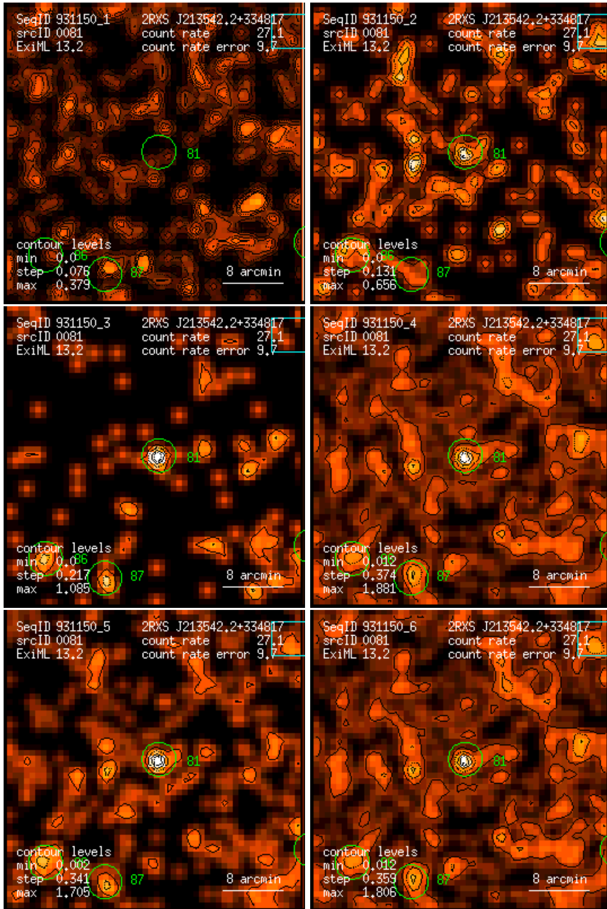
Figure 81: RASS 931150: detection 0081: band rate images, Gaussian filter: (1) PSPC channels 11 – 41, (2) 52 – 90, (3) 91 – 201, (4) 11 – 235, (5) 52 – 201, (6) 11 – 201. Broad band rates in counts/ks. Band rate contour levels in counts/ks/arcmin 2 .
