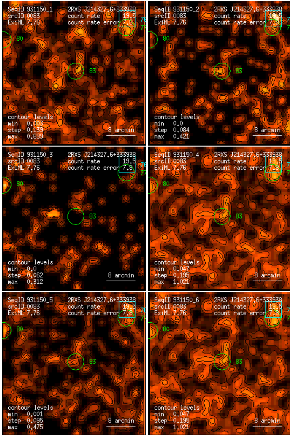
Figure 83: RASS 931150: detection 0083: band rate images, Gaussian filter: (1) PSPC channels 11 – 41, (2) 52 – 90, (3) 91 – 201, (4) 11 – 235, (5) 52 – 201, (6) 11 – 201. Broad band rates in counts/ks. Band rate contour levels in counts/ks/arcmin 2 .
