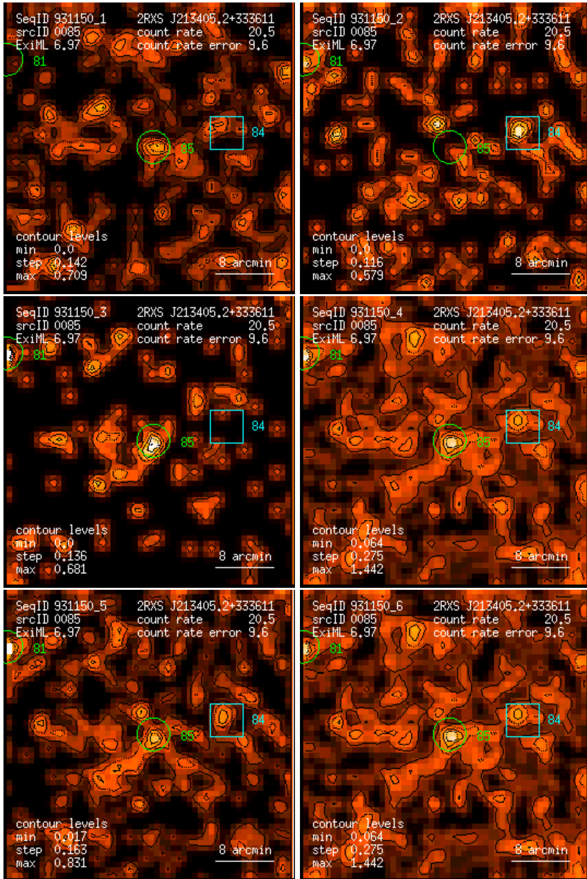
Figure 85: RASS 931150: detection 0085: band rate images, Gaussian filter: (1) PSPC channels 11 – 41, (2) 52 – 90, (3) 91 – 201, (4) 11 – 235, (5) 52 – 201, (6) 11 – 201. Broad band rates in counts/ks. Band rate contour levels in counts/ks/arcmin 2 .
