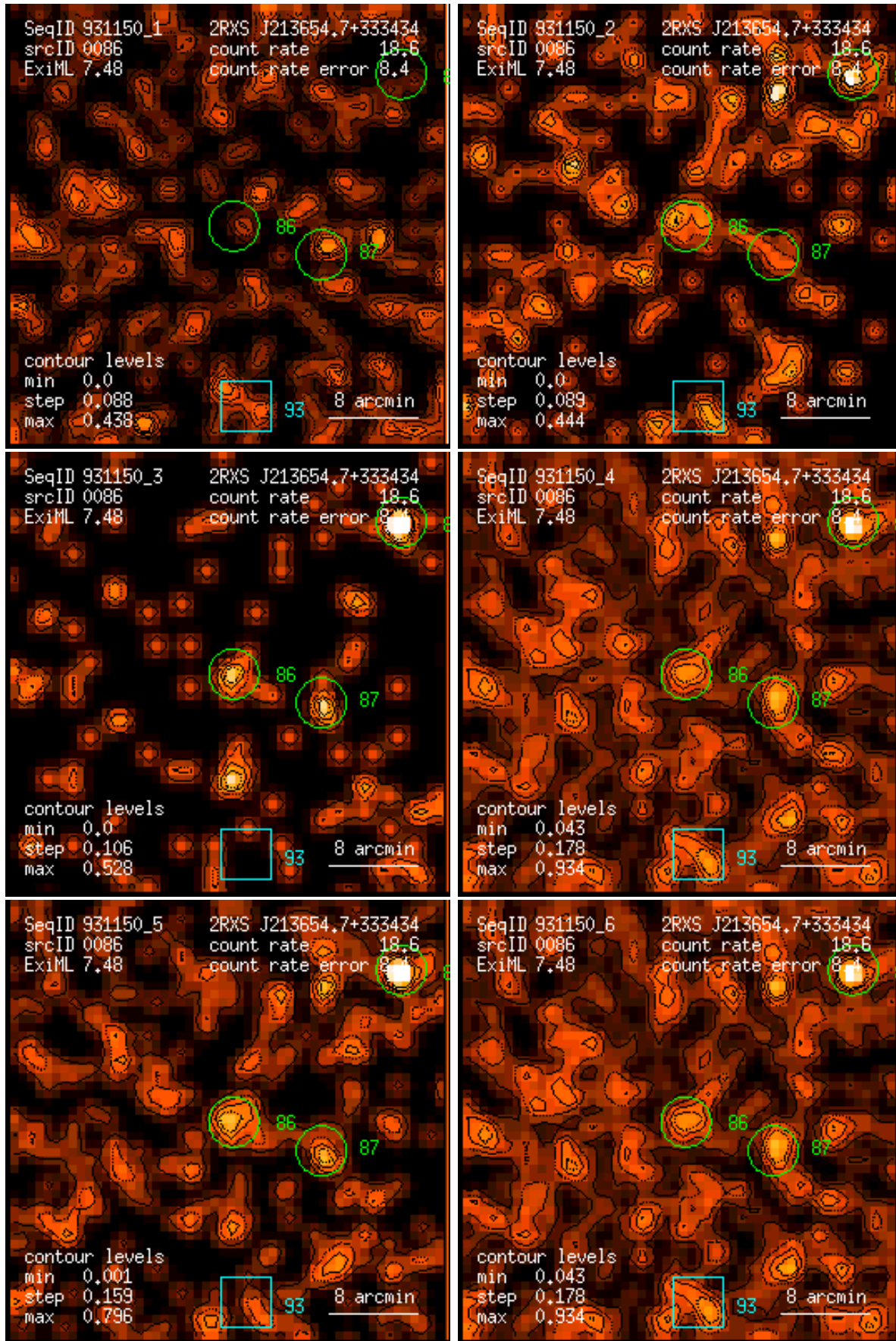
Figure 86: RASS 931150: detection 0086: band rate images, Gaussian filter: (1) PSPC channels 11 – 41, (2) 52 – 90, (3) 91 – 201, (4) 11 – 235, (5) 52 – 201, (6) 11 – 201. Broad band rates in counts/ks. Band rate contour levels in counts/ks/arcmin 2 .
