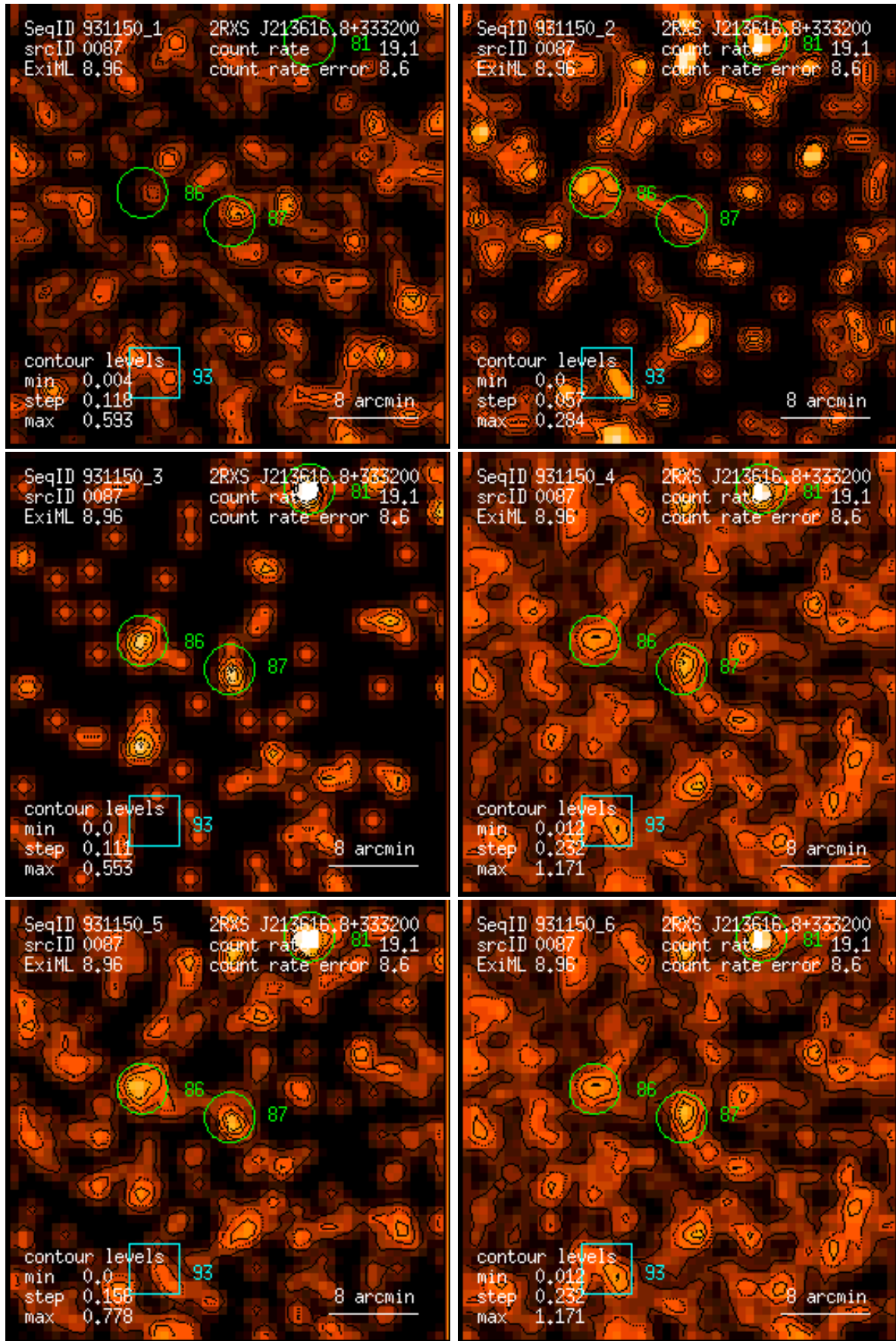
Figure 87: RASS 931150: detection 0087: band rate images, Gaussian filter: (1) PSPC channels 11 – 41, (2) 52 – 90, (3) 91 – 201, (4) 11 – 235, (5) 52 – 201, (6) 11 – 201. Broad band rates in counts/ks. Band rate contour levels in counts/ks/arcmin 2 .
