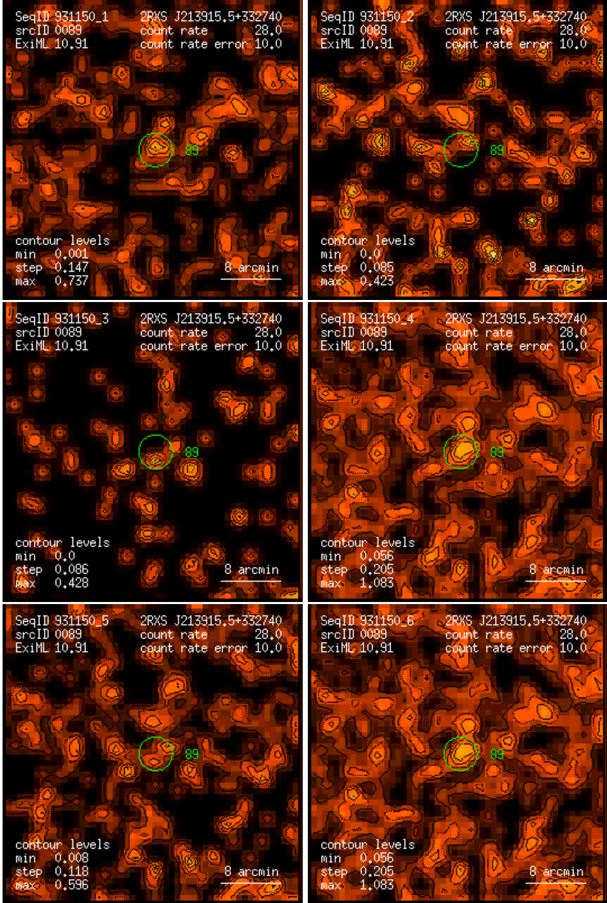
Figure 89: RASS 931150: detection 0089: band rate images, Gaussian filter: (1) PSPC channels 11 – 41, (2) 52 – 90, (3) 91 – 201, (4) 11 – 235, (5) 52 – 201, (6) 11 – 201. Broad band rates in counts/ks. Band rate contour levels in counts/ks/arcmin 2 .
