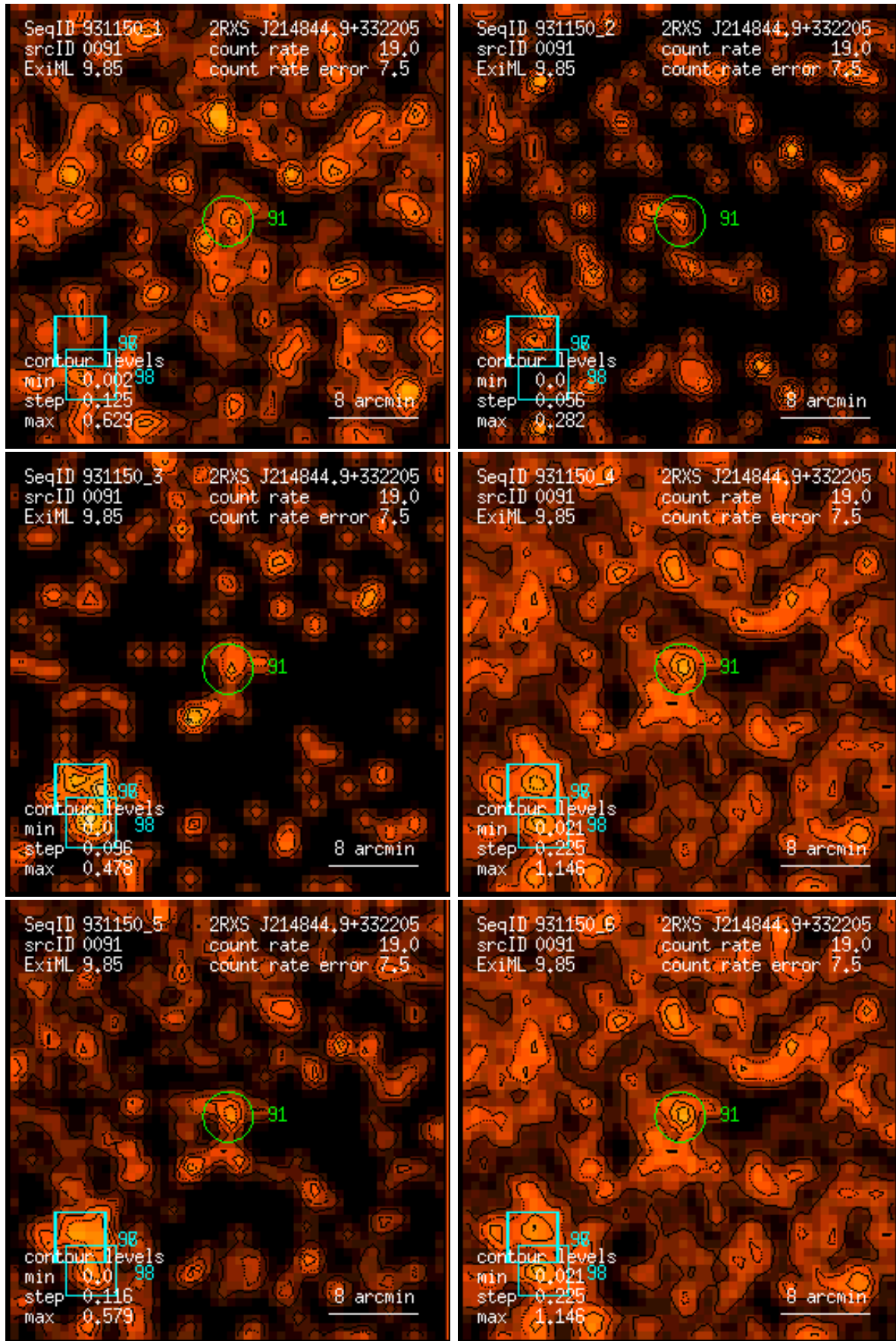
Figure 91: RASS 931150: detection 0091: band rate images, Gaussian filter: (1) PSPC channels 11 – 41, (2) 52 – 90, (3) 91 – 201, (4) 11 – 235, (5) 52 – 201, (6) 11 – 201. Broad band rates in counts/ks. Band rate contour levels in counts/ks/arcmin 2 .
