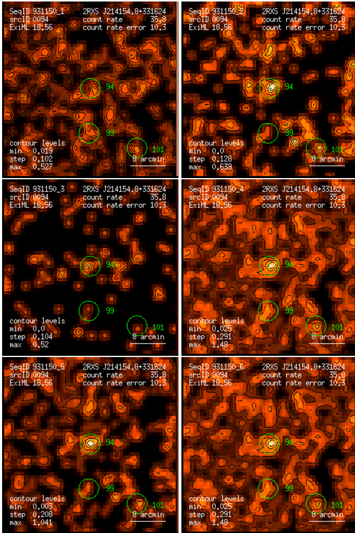
Figure 94: RASS 931150: detection 0094: band rate images, Gaussian filter: (1) PSPC channels 11 – 41, (2) 52 – 90, (3) 91 – 201, (4) 11 – 235, (5) 52 – 201, (6) 11 – 201. Broad band rates in counts/ks. Band rate contour levels in counts/ks/arcmin 2 .
