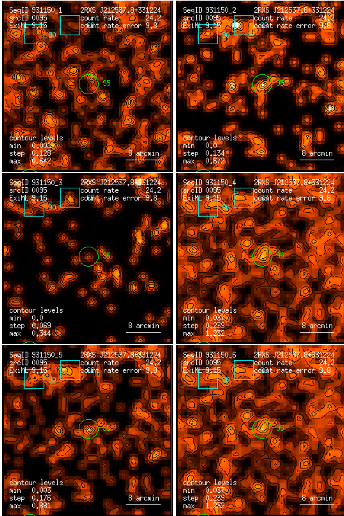
Figure 95: RASS 931150: detection 0095: band rate images, Gaussian filter: (1) PSPC channels 11 – 41, (2) 52 – 90, (3) 91 – 201, (4) 11 – 235, (5) 52 – 201, (6) 11 – 201. Broad band rates in counts/ks. Band rate contour levels in counts/ks/arcmin 2 .
