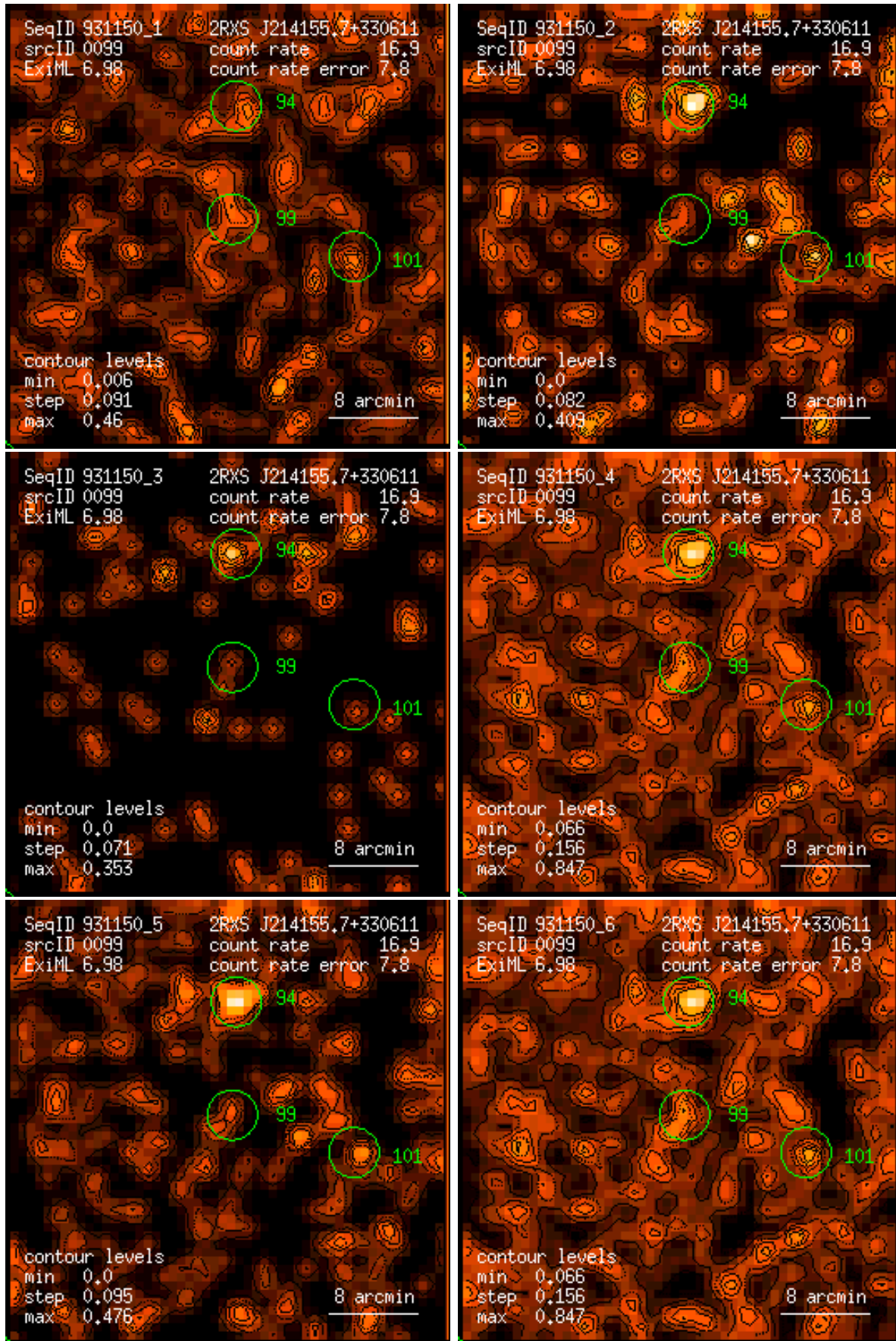
Figure 99: RASS 931150: detection 0099: band rate images, Gaussian filter: (1) PSPC channels 11 – 41, (2) 52 – 90, (3) 91 – 201, (4) 11 – 235, (5) 52 – 201, (6) 11 – 201. Broad band rates in counts/ks. Band rate contour levels in counts/ks/arcmin 2 .
