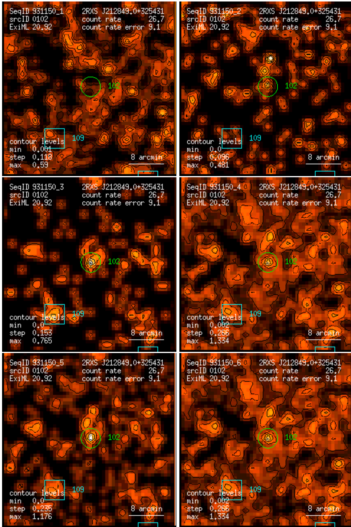
Figure 102: RASS 931150: detection 0102: band rate images, Gaussian filter: (1) PSPC channels 11 – 41, (2) 52 – 90, (3) 91 – 201, (4) 11 – 235, (5) 52 – 201, (6) 11 – 201. Broad band rates in counts/ks. Band rate contour levels in counts/ks/arcmin 2 .
