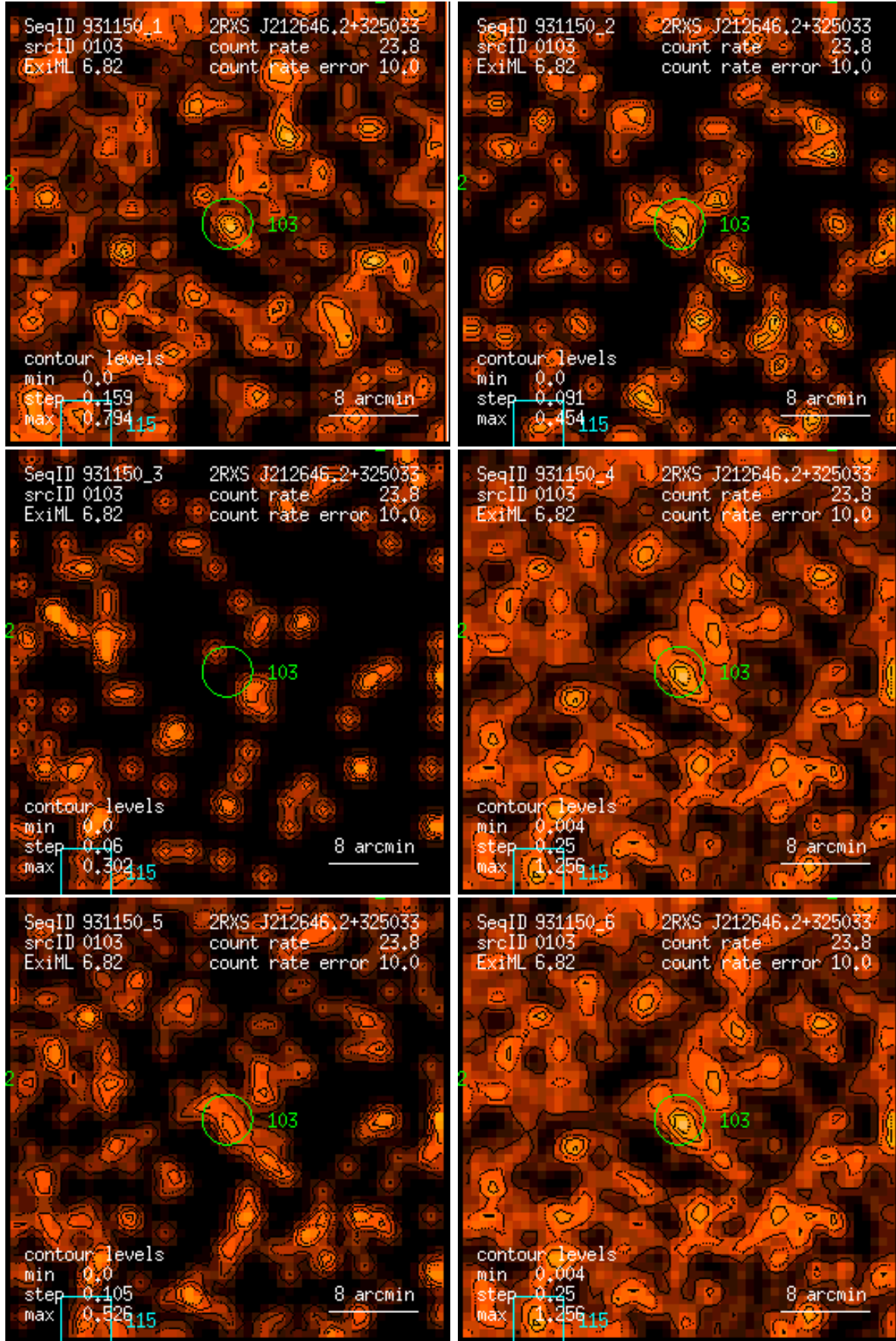
Figure 103: RASS 931150: detection 0103: band rate images, Gaussian filter: (1) PSPC channels 11 – 41, (2) 52 – 90, (3) 91 – 201, (4) 11 – 235, (5) 52 – 201, (6) 11 – 201. Broad band rates in counts/ks. Band rate contour levels in counts/ks/arcmin 2 .
