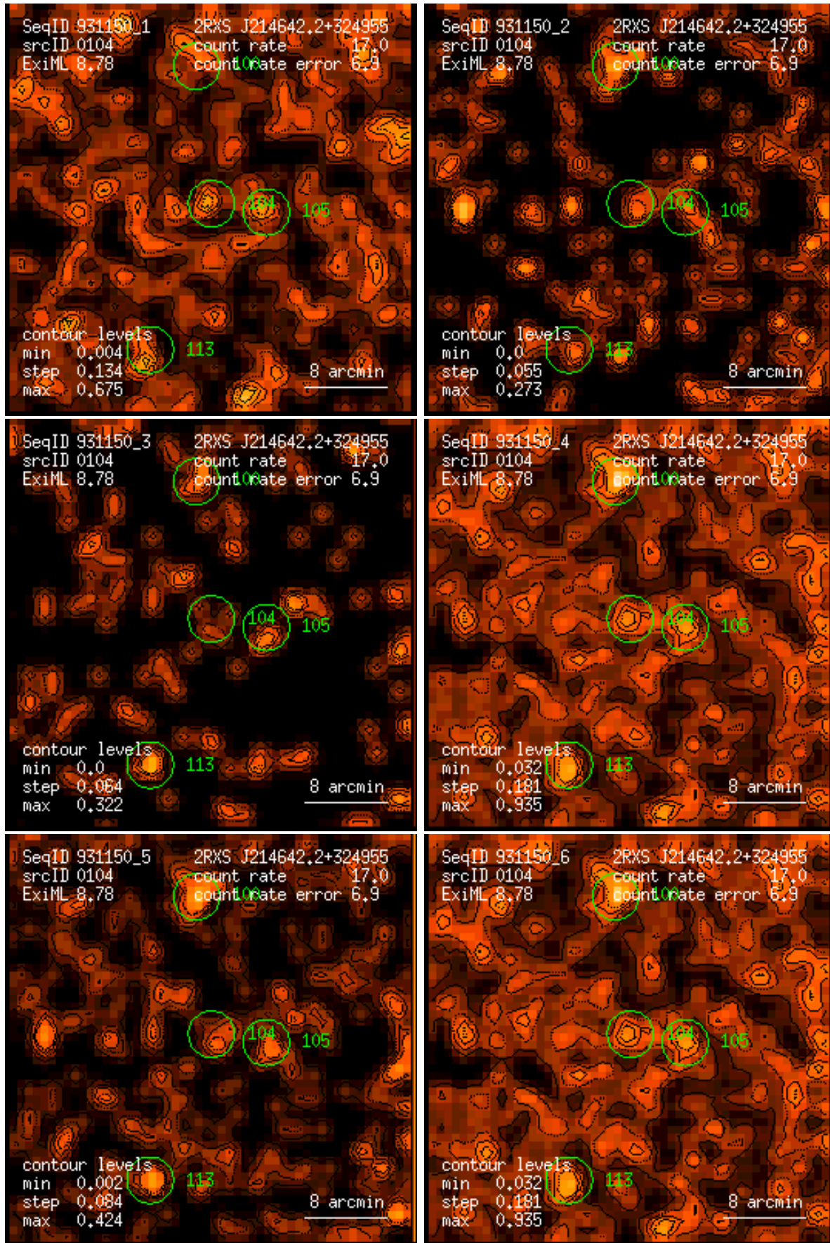
Figure 104: RASS 931150: detection 0104: band rate images, Gaussian filter: (1) PSPC channels 11 – 41, (2) 52 – 90, (3) 91 – 201, (4) 11 – 235, (5) 52 – 201, (6) 11 – 201. Broad band rates in counts/ks. Band rate contour levels in counts/ks/arcmin 2 .
