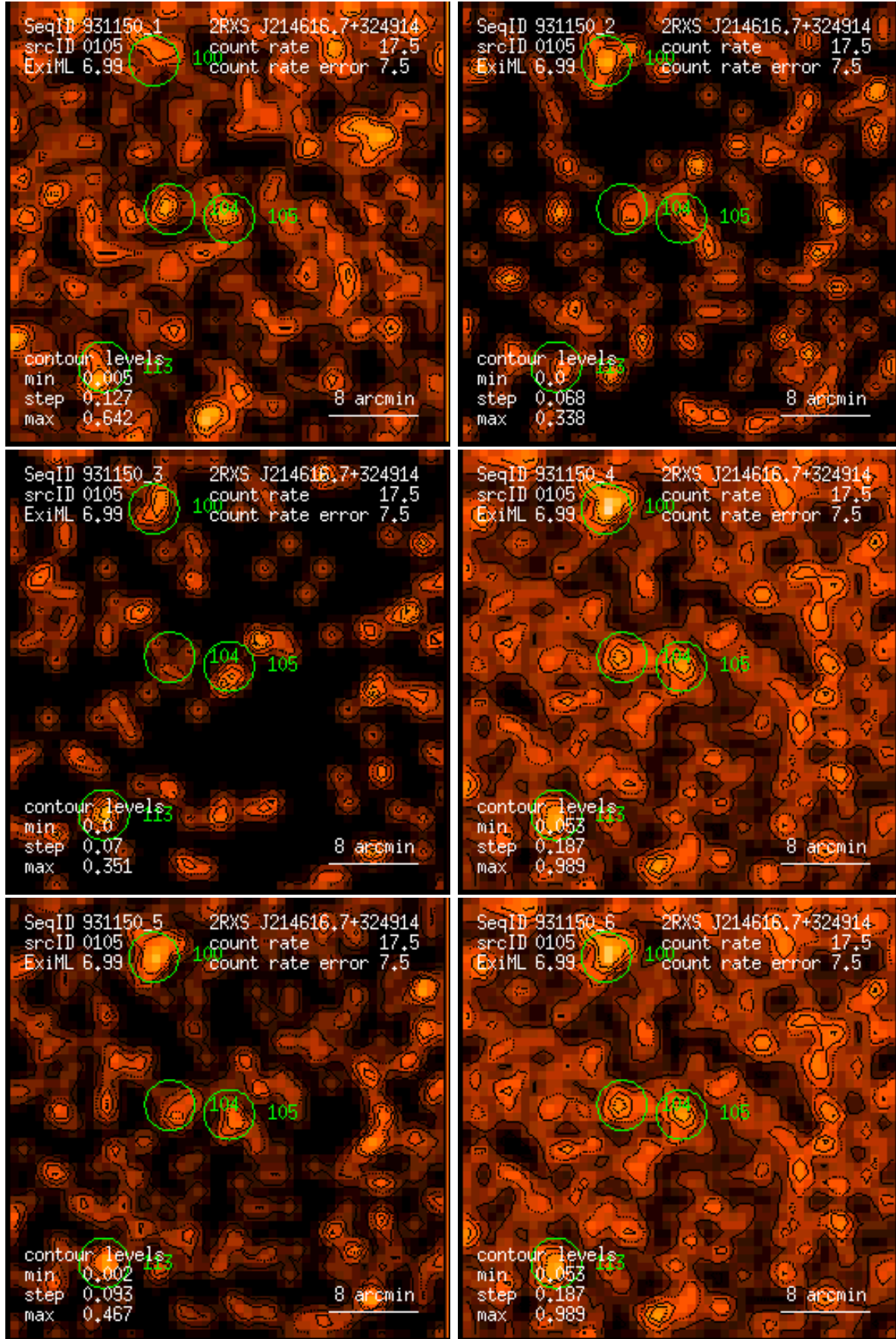
Figure 105: RASS 931150: detection 0105: band rate images, Gaussian filter: (1) PSPC channels 11 – 41, (2) 52 – 90, (3) 91 – 201, (4) 11 – 235, (5) 52 – 201, (6) 11 – 201. Broad band rates in counts/ks. Band rate contour levels in counts/ks/arcmin 2 .
