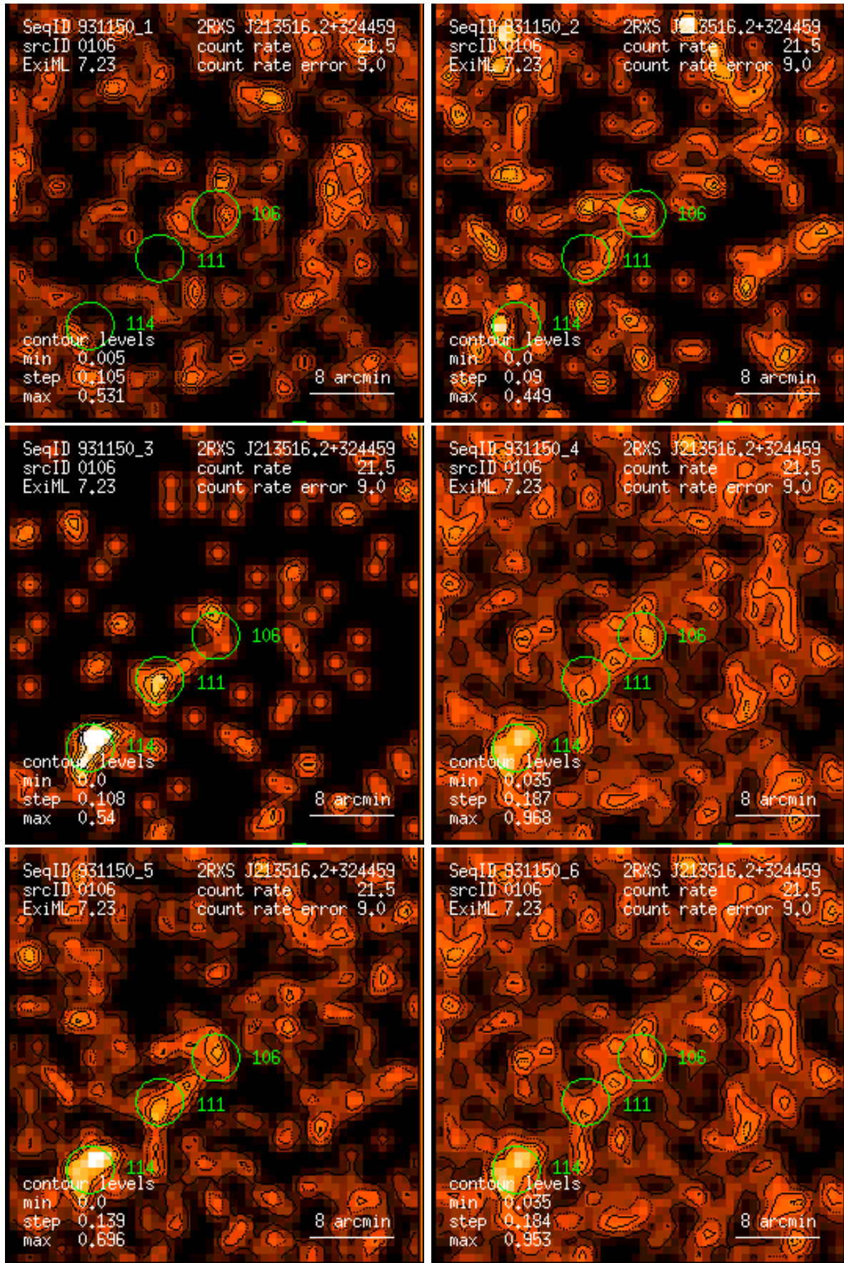
Figure 106: RASS 931150: detection 0106: band rate images, Gaussian filter: (1) PSPC channels 11 – 41, (2) 52 – 90, (3) 91 – 201, (4) 11 – 235, (5) 52 – 201, (6) 11 – 201. Broad band rates in counts/ks. Band rate contour levels in counts/ks/arcmin 2 .
