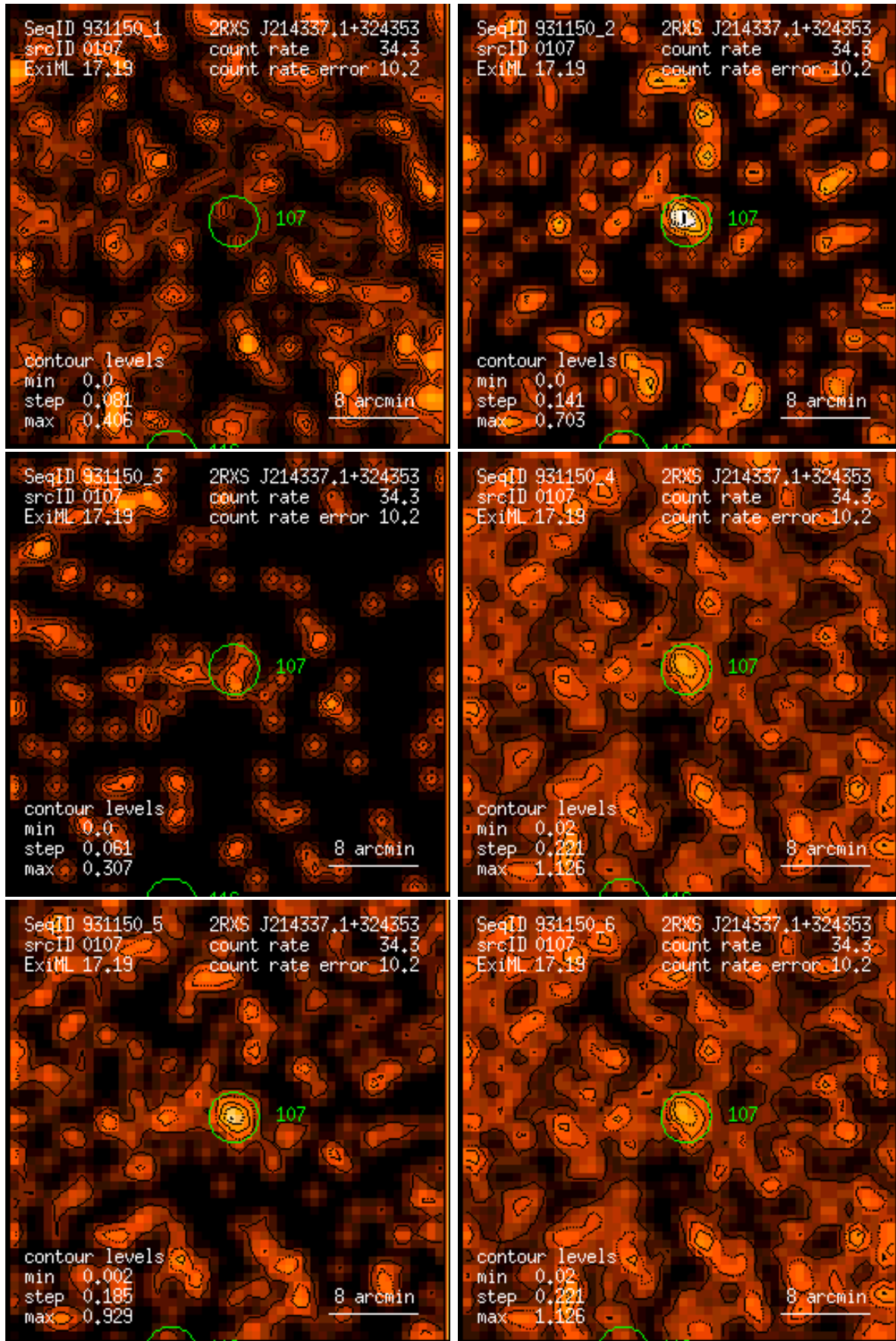
Figure 107: RASS 931150: detection 0107: band rate images, Gaussian filter: (1) PSPC channels 11 – 41, (2) 52 – 90, (3) 91 – 201, (4) 11 – 235, (5) 52 – 201, (6) 11 – 201. Broad band rates in counts/ks. Band rate contour levels in counts/ks/arcmin 2 .
