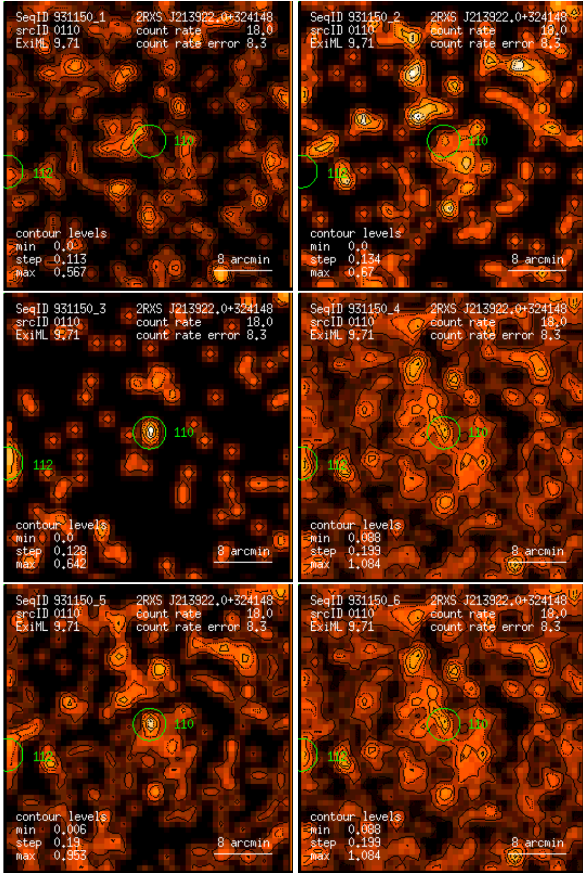
Figure 110: RASS 931150: detection 0110: band rate images, Gaussian filter: (1) PSPC channels 11 – 41, (2) 52 – 90, (3) 91 – 201, (4) 11 – 235, (5) 52 – 201, (6) 11 – 201. Broad band rates in counts/ks. Band rate contour levels in counts/ks/arcmin 2 .
