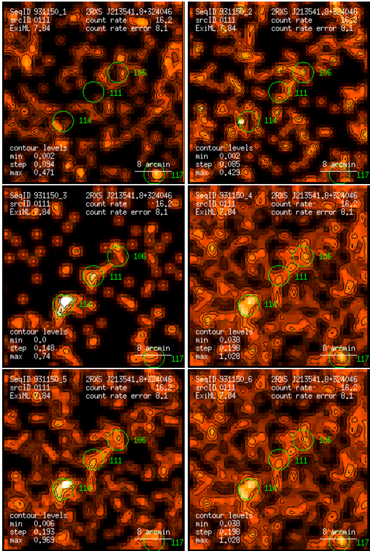
Figure 111: RASS 931150: detection 0111: band rate images, Gaussian filter: (1) PSPC channels 11 – 41, (2) 52 – 90, (3) 91 – 201, (4) 11 – 235, (5) 52 – 201, (6) 11 – 201. Broad band rates in counts/ks. Band rate contour levels in counts/ks/arcmin 2 .
