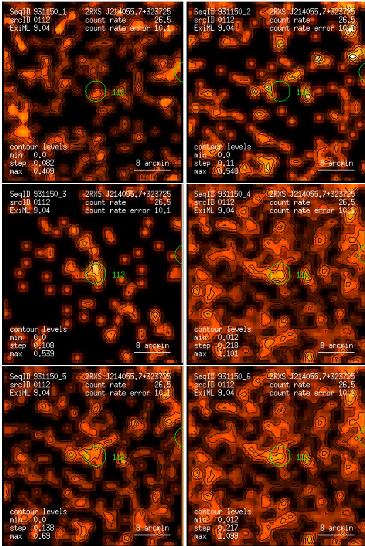
Figure 112: RASS 931150: detection 0112: band rate images, Gaussian filter: (1) PSPC channels 11 – 41, (2) 52 – 90, (3) 91 – 201, (4) 11 – 235, (5) 52 – 201, (6) 11 – 201. Broad band rates in counts/ks. Band rate contour levels in counts/ks/arcmin 2 .
