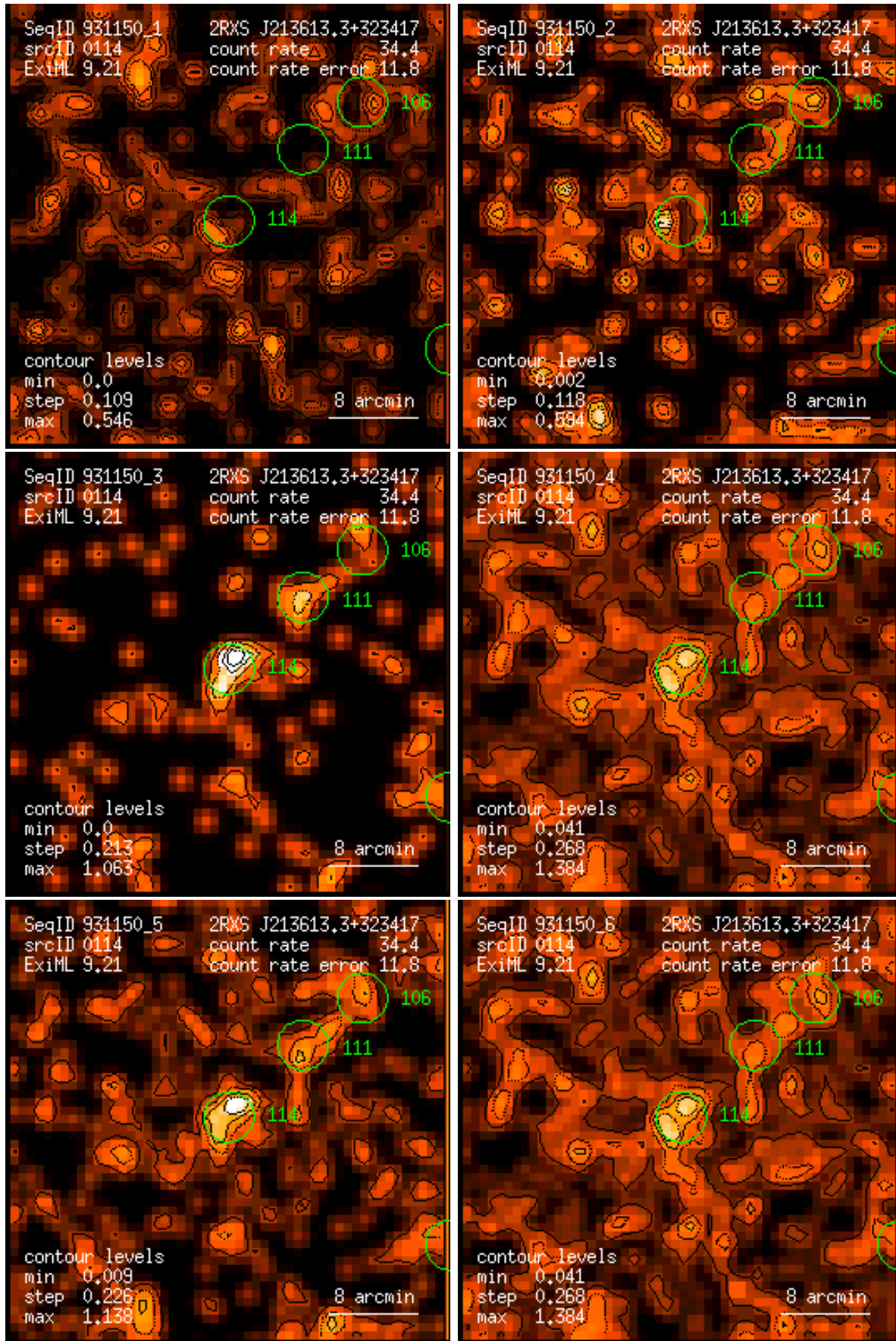
Figure 114: RASS 931150: detection 0114: band rate images, Gaussian filter: (1) PSPC channels 11 – 41, (2) 52 – 90, (3) 91 – 201, (4) 11 – 235, (5) 52 – 201, (6) 11 – 201. Broad band rates in counts/ks. Band rate contour levels in counts/ks/arcmin 2 .
