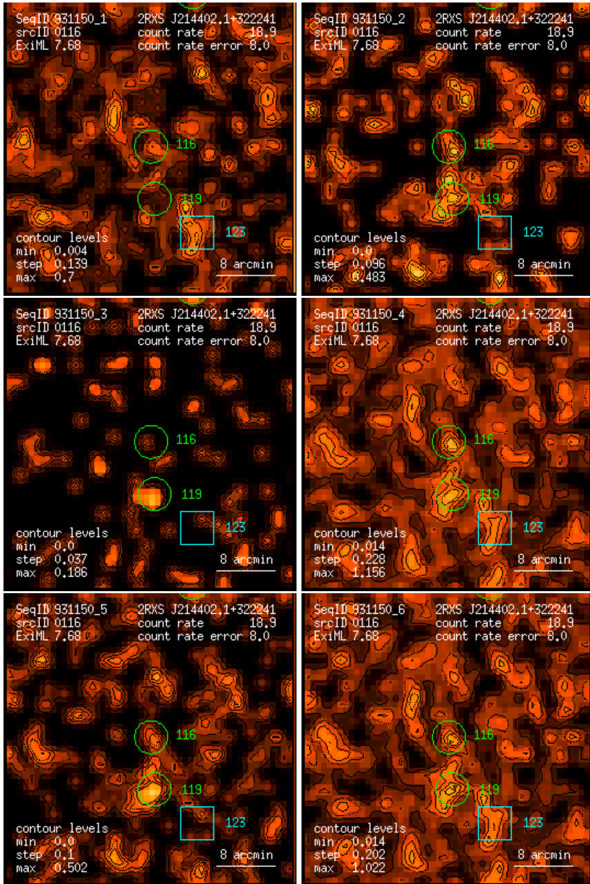
Figure 116: RASS 931150: detection 0116: band rate images, Gaussian filter: (1) PSPC channels 11 – 41, (2) 52 – 90, (3) 91 – 201, (4) 11 – 235, (5) 52 – 201, (6) 11 – 201. Broad band rates in counts/ks. Band rate contour levels in counts/ks/arcmin 2 .
