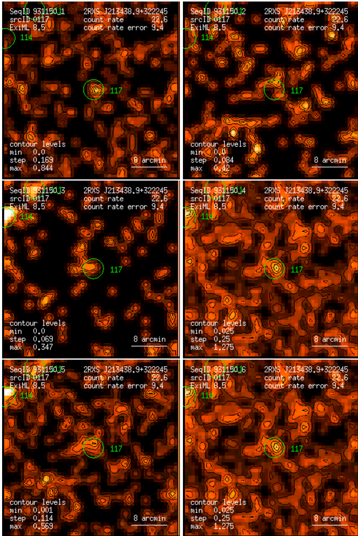
Figure 117: RASS 931150: detection 0117: band rate images, Gaussian filter: (1) PSPC channels 11 – 41, (2) 52 – 90, (3) 91 – 201, (4) 11 – 235, (5) 52 – 201, (6) 11 – 201. Broad band rates in counts/ks. Band rate contour levels in counts/ks/arcmin 2 .
