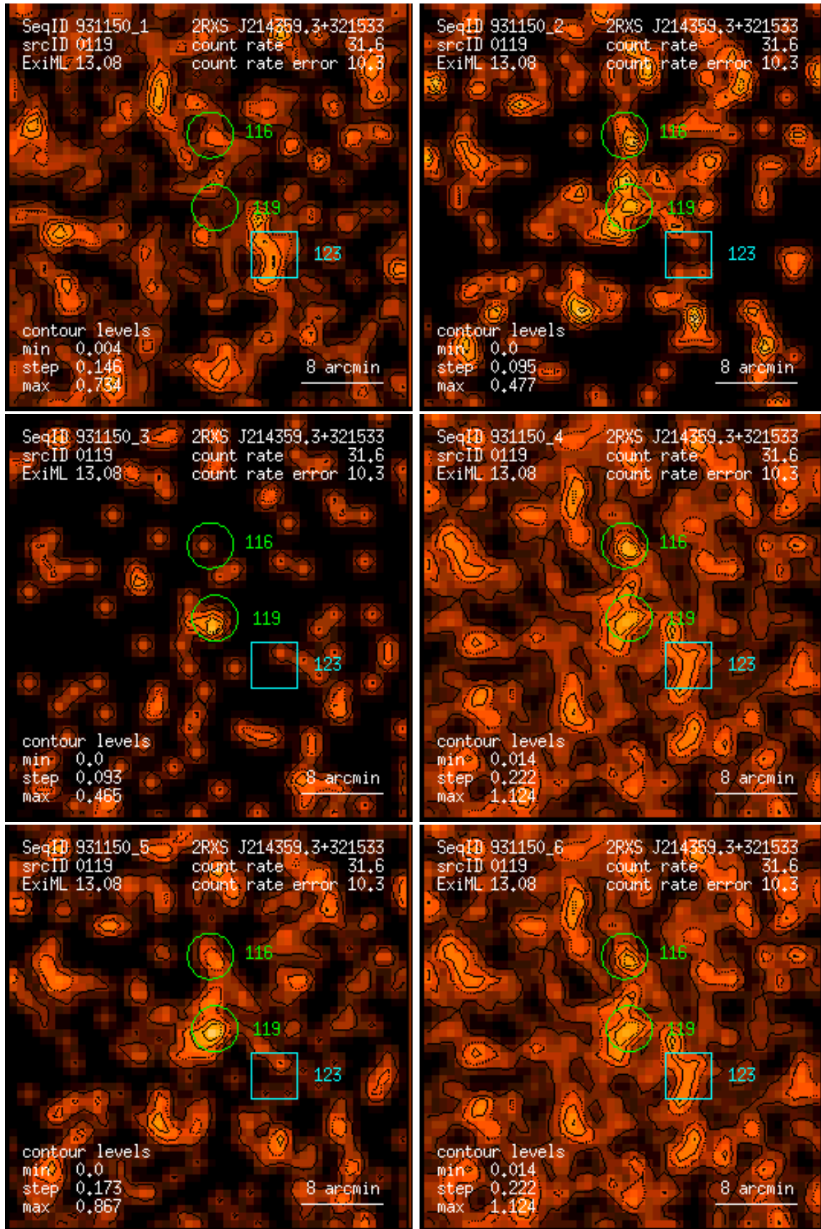
Figure 119: RASS 931150: detection 0119: band rate images, Gaussian filter: (1) PSPC channels 11 – 41, (2) 52 – 90, (3) 91 – 201, (4) 11 – 235, (5) 52 – 201, (6) 11 – 201. Broad band rates in counts/ks. Band rate contour levels in counts/ks/arcmin 2 .
