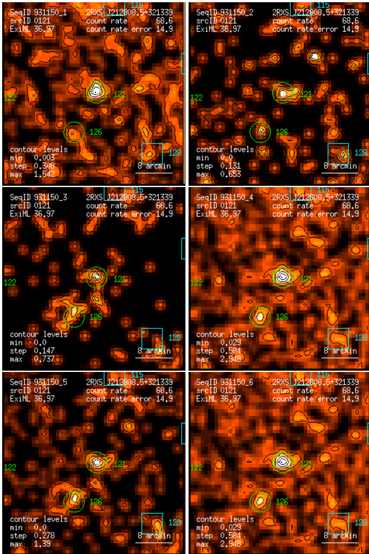
Figure 121: RASS 931150: detection 0121: band rate images, Gaussian filter: (1) PSPC channels 11 – 41, (2) 52 – 90, (3) 91 – 201, (4) 11 – 235, (5) 52 – 201, (6) 11 – 201. Broad band rates in counts/ks. Band rate contour levels in counts/ks/arcmin 2 .
