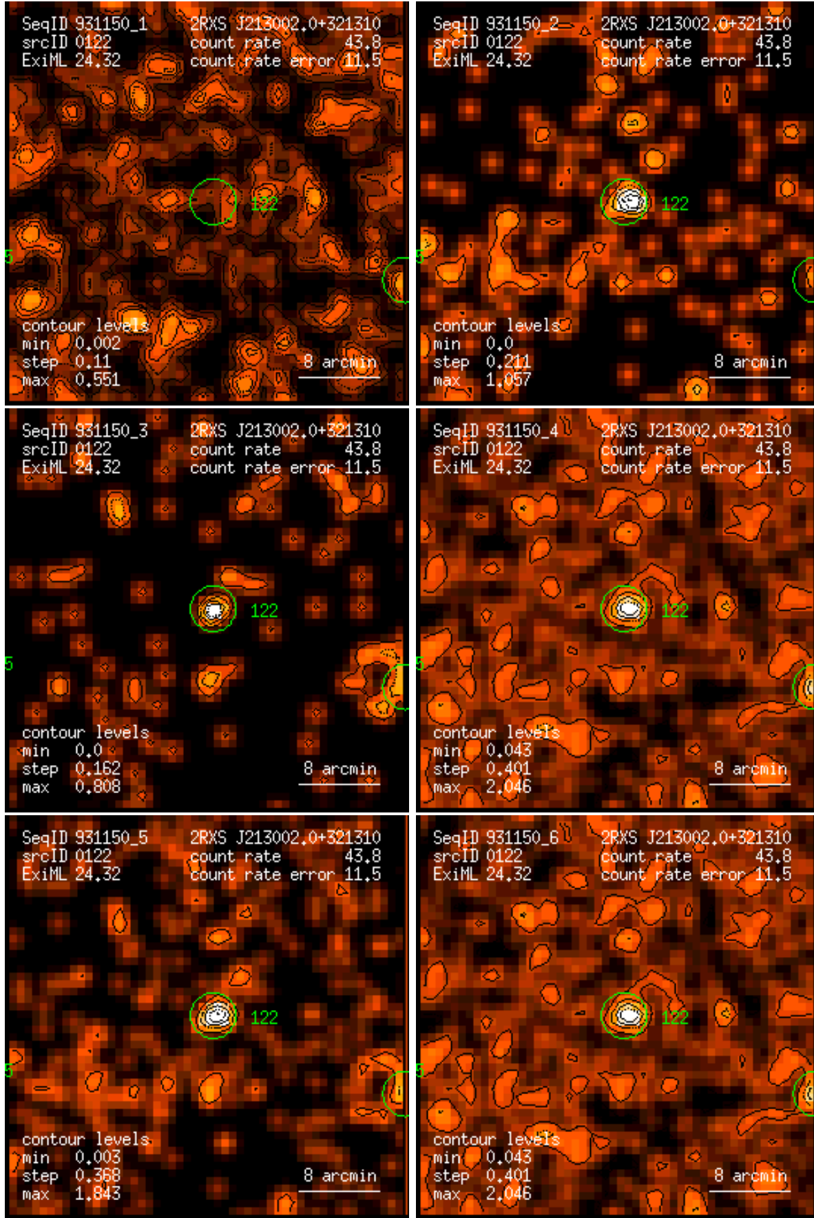
Figure 122: RASS 931150: detection 0122: band rate images, Gaussian filter: (1) PSPC channels 11 – 41, (2) 52 – 90, (3) 91 – 201, (4) 11 – 235, (5) 52 – 201, (6) 11 – 201. Broad band rates in counts/ks. Band rate contour levels in counts/ks/arcmin 2 .
