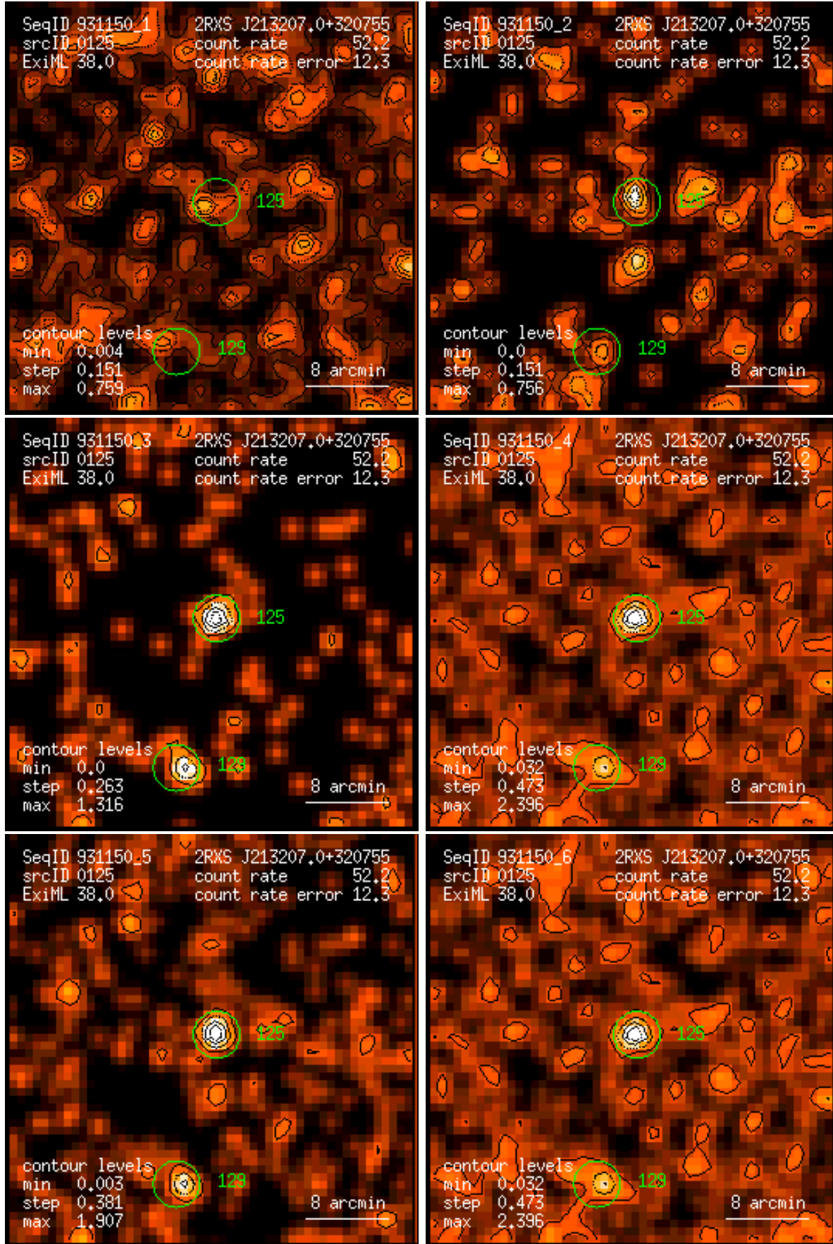
Figure 125: RASS 931150: detection 0125: band rate images, Gaussian filter: (1) PSPC channels 11 – 41, (2) 52 – 90, (3) 91 – 201, (4) 11 – 235, (5) 52 – 201, (6) 11 – 201. Broad band rates in counts/ks. Band rate contour levels in counts/ks/arcmin 2 .
