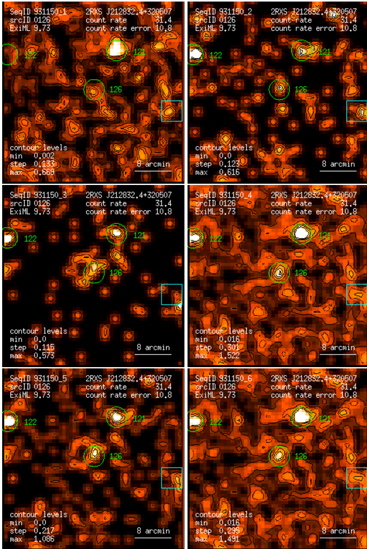
Figure 126: RASS 931150: detection 0126: band rate images, Gaussian filter: (1) PSPC channels 11 – 41, (2) 52 – 90, (3) 91 – 201, (4) 11 – 235, (5) 52 – 201, (6) 11 – 201. Broad band rates in counts/ks. Band rate contour levels in counts/ks/arcmin 2 .
