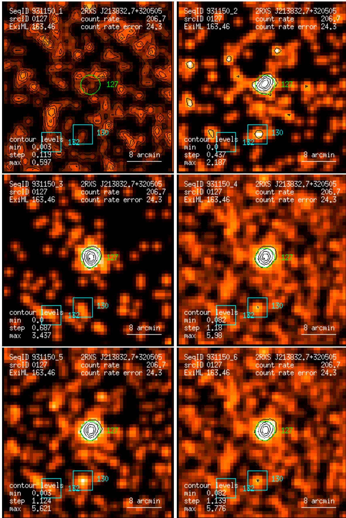
Figure 127: RASS 931150: detection 0127: band rate images, Gaussian filter: (1) PSPC channels 11 – 41, (2) 52 – 90, (3) 91 – 201, (4) 11 – 235, (5) 52 – 201, (6) 11 – 201. Broad band rates in counts/ks. Band rate contour levels in counts/ks/arcmin 2 .
