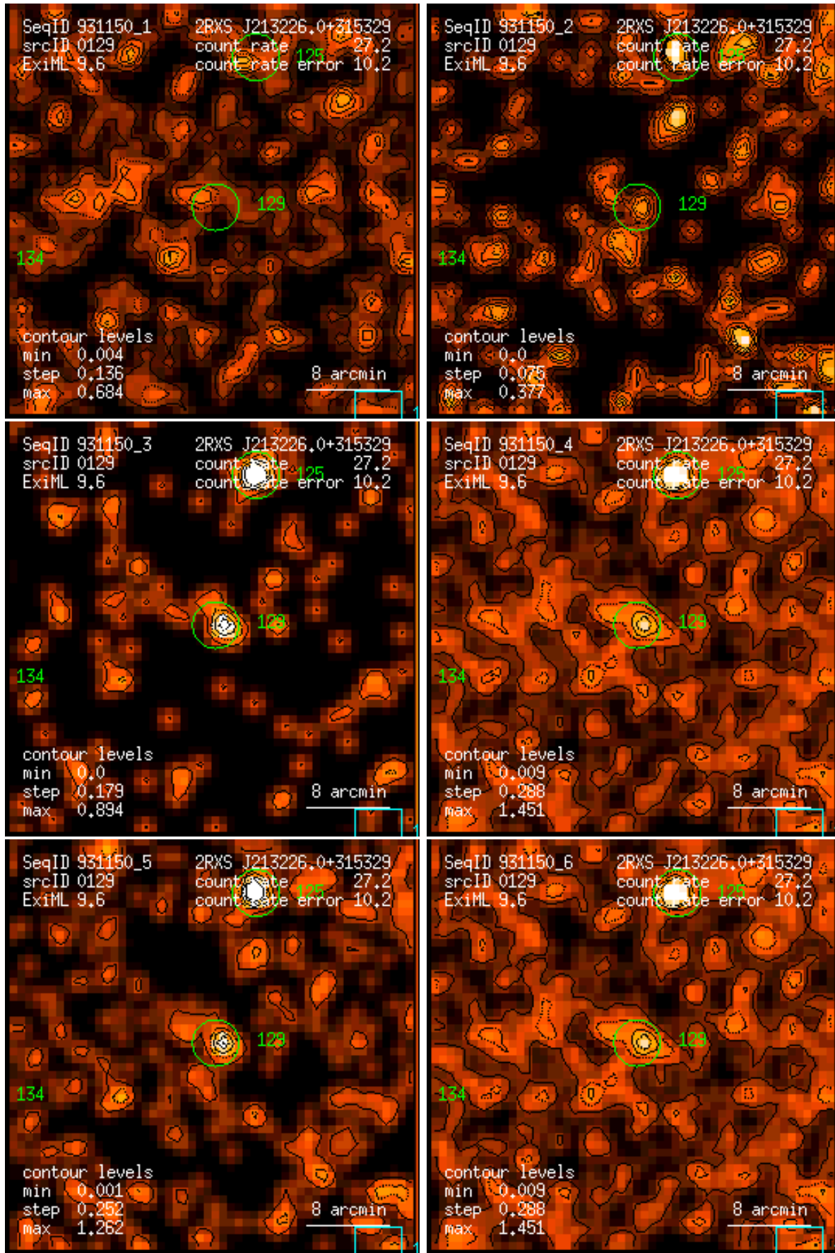
Figure 129: RASS 931150: detection 0129: band rate images, Gaussian filter: (1) PSPC channels 11 – 41, (2) 52 – 90, (3) 91 – 201, (4) 11 – 235, (5) 52 – 201, (6) 11 – 201. Broad band rates in counts/ks. Band rate contour levels in counts/ks/arcmin 2 .
