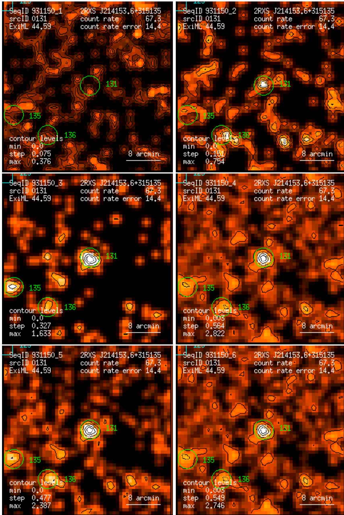
Figure 131: RASS 931150: detection 0131: band rate images, Gaussian filter: (1) PSPC channels 11 – 41, (2) 52 – 90, (3) 91 – 201, (4) 11 – 235, (5) 52 – 201, (6) 11 – 201. Broad band rates in counts/ks. Band rate contour levels in counts/ks/arcmin 2 .
