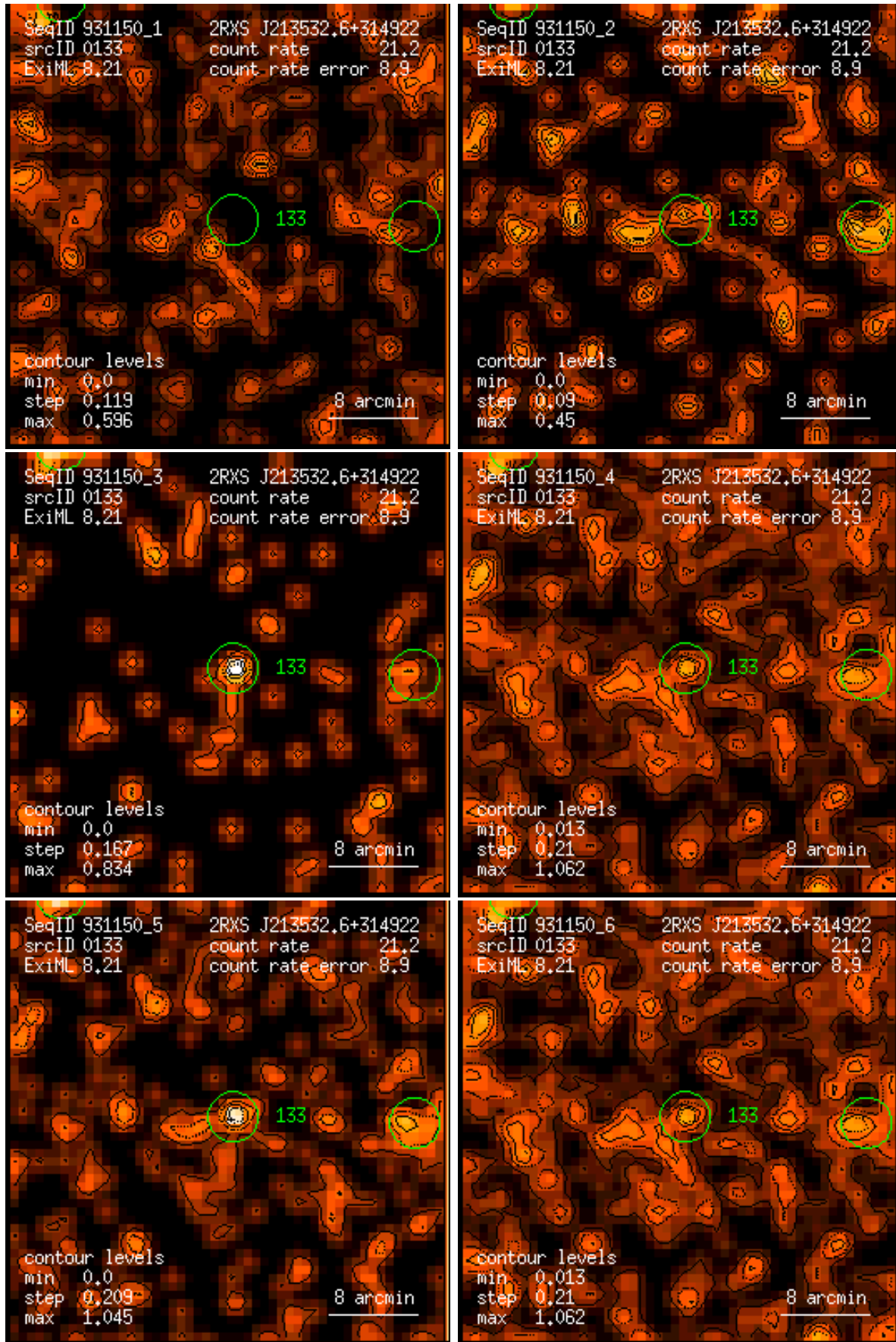
Figure 133: RASS 931150: detection 0133: band rate images, Gaussian filter: (1) PSPC channels 11 – 41, (2) 52 – 90, (3) 91 – 201, (4) 11 – 235, (5) 52 – 201, (6) 11 – 201. Broad band rates in counts/ks. Band rate contour levels in counts/ks/arcmin 2 .
