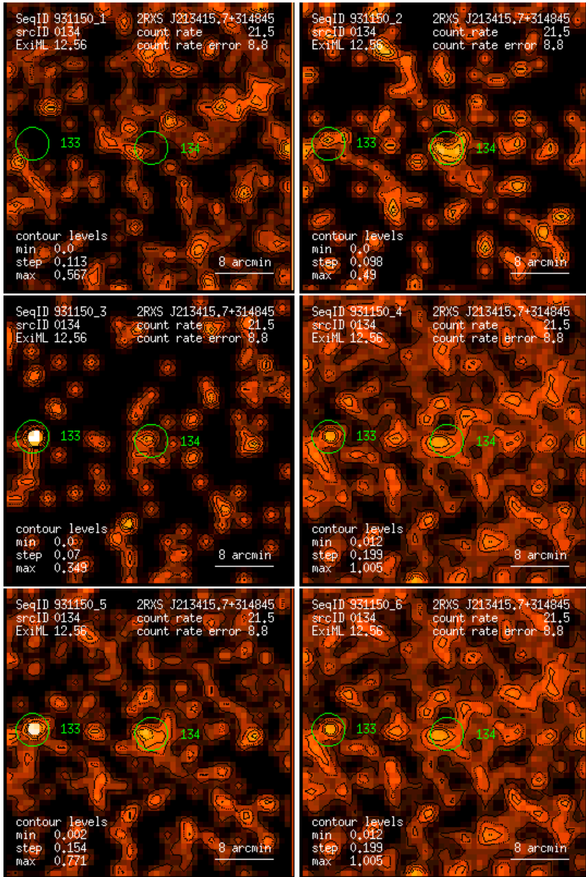
Figure 134: RASS 931150: detection 0134: band rate images, Gaussian filter: (1) PSPC channels 11 – 41, (2) 52 – 90, (3) 91 – 201, (4) 11 – 235, (5) 52 – 201, (6) 11 – 201. Broad band rates in counts/ks. Band rate contour levels in counts/ks/arcmin 2 .
