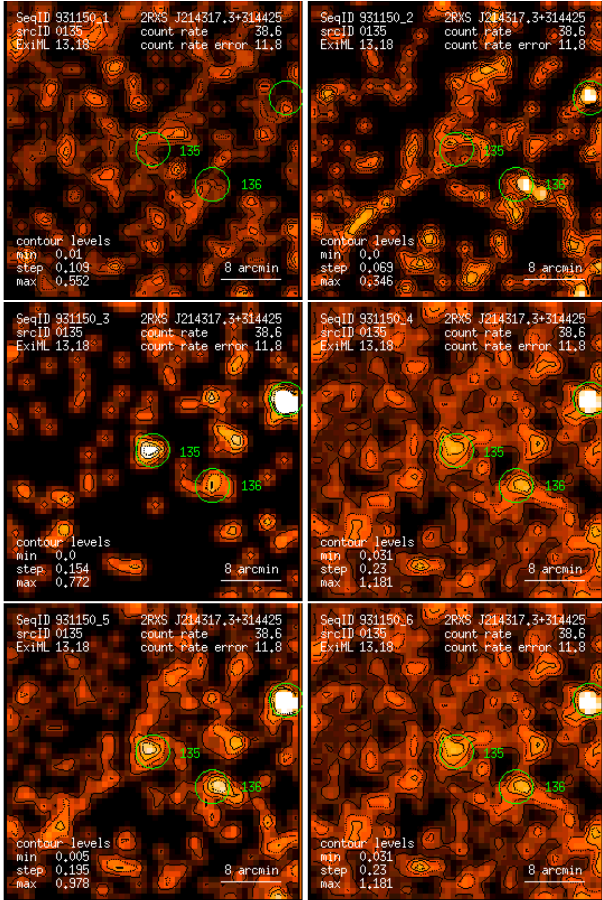
Figure 135: RASS 931150: detection 0135: band rate images, Gaussian filter: (1) PSPC channels 11 – 41, (2) 52 – 90, (3) 91 – 201, (4) 11 – 235, (5) 52 – 201, (6) 11 – 201. Broad band rates in counts/ks. Band rate contour levels in counts/ks/arcmin 2 .
