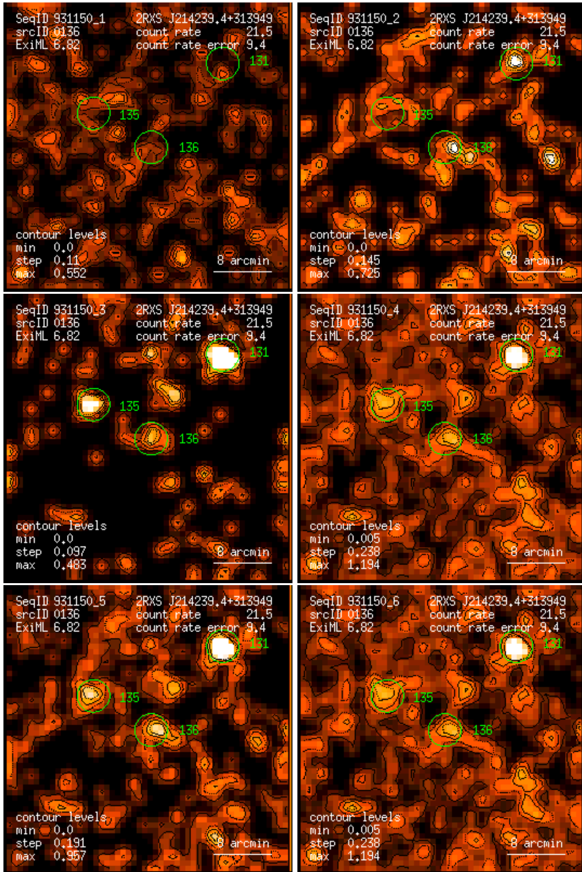
Figure 136: RASS 931150: detection 0136: band rate images, Gaussian filter: (1) PSPC channels 11 – 41, (2) 52 – 90, (3) 91 – 201, (4) 11 – 235, (5) 52 – 201, (6) 11 – 201. Broad band rates in counts/ks. Band rate contour levels in counts/ks/arcmin 2 .
