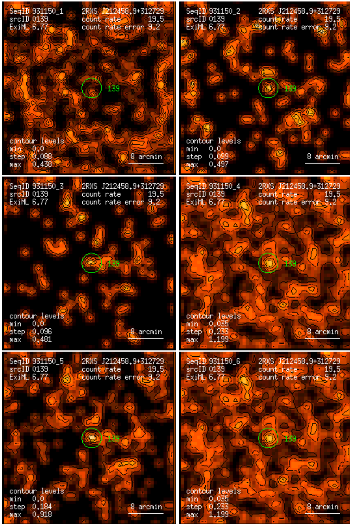
Figure 139: RASS 931150: detection 0139: band rate images, Gaussian filter: (1) PSPC channels 11 – 41, (2) 52 – 90, (3) 91 – 201, (4) 11 – 235, (5) 52 – 201, (6) 11 – 201. Broad band rates in counts/ks. Band rate contour levels in counts/ks/arcmin 2 .
