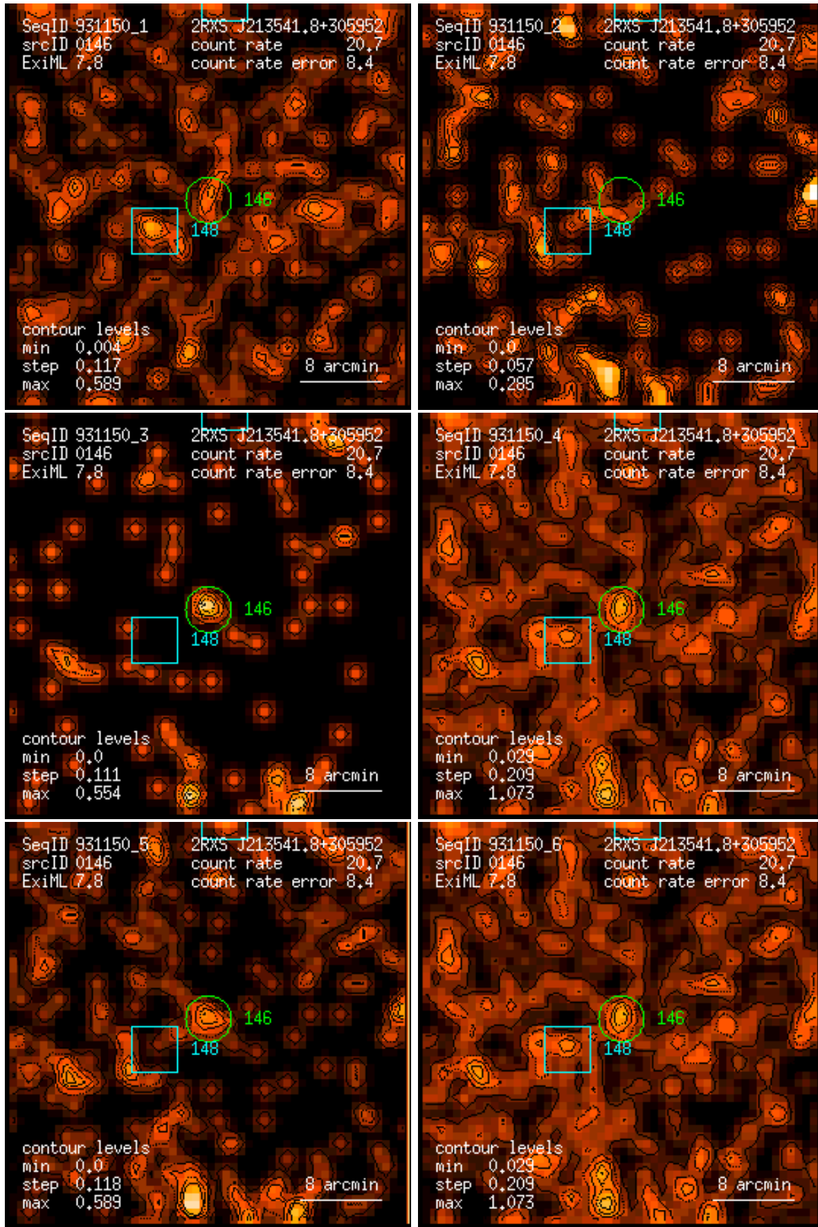
Figure 146: RASS 931150: detection 0146: band rate images, Gaussian filter: (1) PSPC channels 11 – 41, (2) 52 – 90, (3) 91 – 201, (4) 11 – 235, (5) 52 – 201, (6) 11 – 201. Broad band rates in counts/ks. Band rate contour levels in counts/ks/arcmin 2 .
