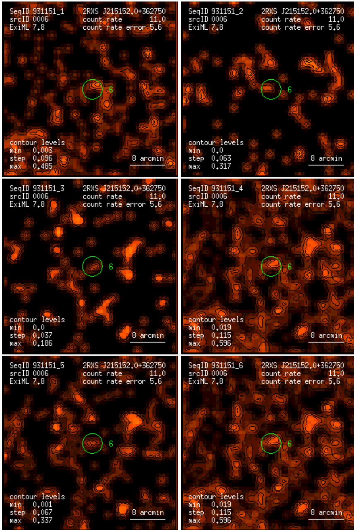
Figure 6: RASS 931151: detection 0006: band rate images, Gaussian filter: (1) PSPC channels 11 – 41, (2) 52 – 90, (3) 91 – 201, (4) 11 – 235, (5) 52 – 201, (6) 11 – 201. Broad band rates in counts/ks. Band rate contour levels in counts/ks/arcmin 2 .
