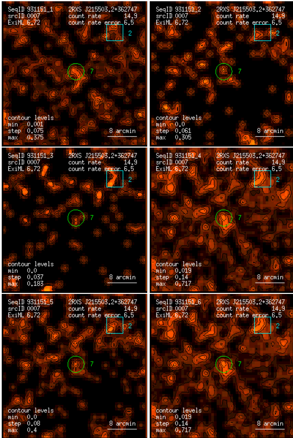
Figure 7: RASS 931151: detection 0007: band rate images, Gaussian filter: (1) PSPC channels 11 – 41, (2) 52 – 90, (3) 91 – 201, (4) 11 – 235, (5) 52 – 201, (6) 11 – 201. Broad band rates in counts/ks. Band rate contour levels in counts/ks/arcmin 2 .
