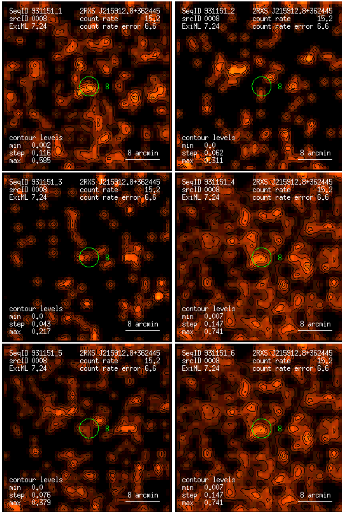
Figure 8: RASS 931151: detection 0008: band rate images, Gaussian filter: (1) PSPC channels 11 – 41, (2) 52 – 90, (3) 91 – 201, (4) 11 – 235, (5) 52 – 201, (6) 11 – 201. Broad band rates in counts/ks. Band rate contour levels in counts/ks/arcmin 2 .
