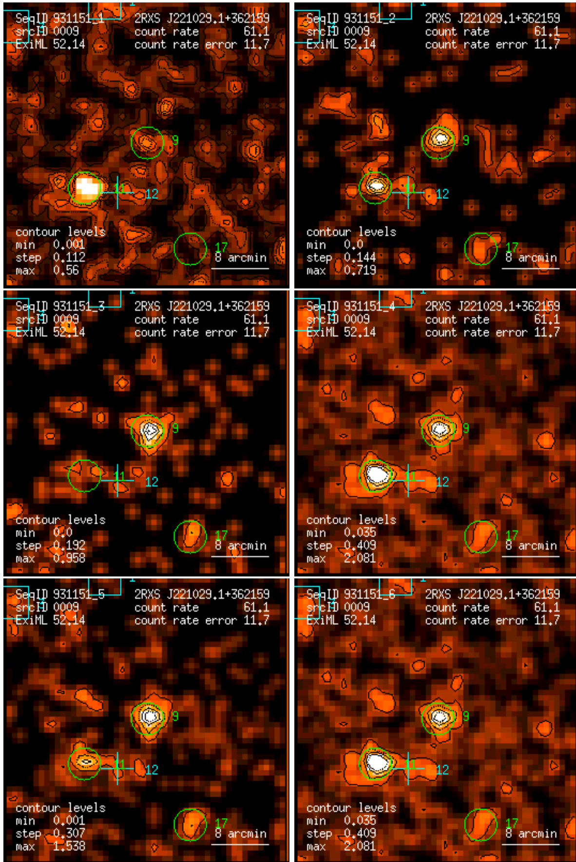
Figure 9: RASS 931151: detection 0009: band rate images, Gaussian filter: (1) PSPC channels 11 – 41, (2) 52 – 90, (3) 91 – 201, (4) 11 – 235, (5) 52 – 201, (6) 11 – 201. Broad band rates in counts/ks. Band rate contour levels in counts/ks/arcmin 2 .
