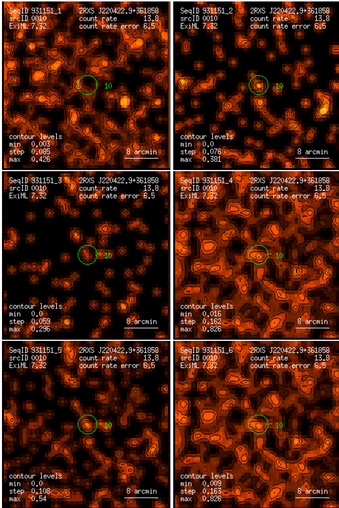
Figure 10: RASS 931151: detection 0010: band rate images, Gaussian filter: (1) PSPC channels 11 – 41, (2) 52 – 90, (3) 91 – 201, (4) 11 – 235, (5) 52 – 201, (6) 11 – 201. Broad band rates in counts/ks. Band rate contour levels in counts/ks/arcmin 2 .
